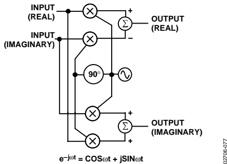
Figure 77. Implementation of a Complex Modulator
