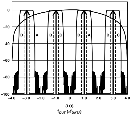
Figure 84. 4x Interpolation, Complex f_{DAC}/4 Modulation
