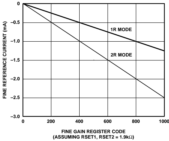
Figure 40. Fine Gain Effect on I_{FULLSCALE}
