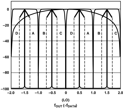
Figure 83. 2x Interpolation, Complex f_{DAC}/4 Modulation
