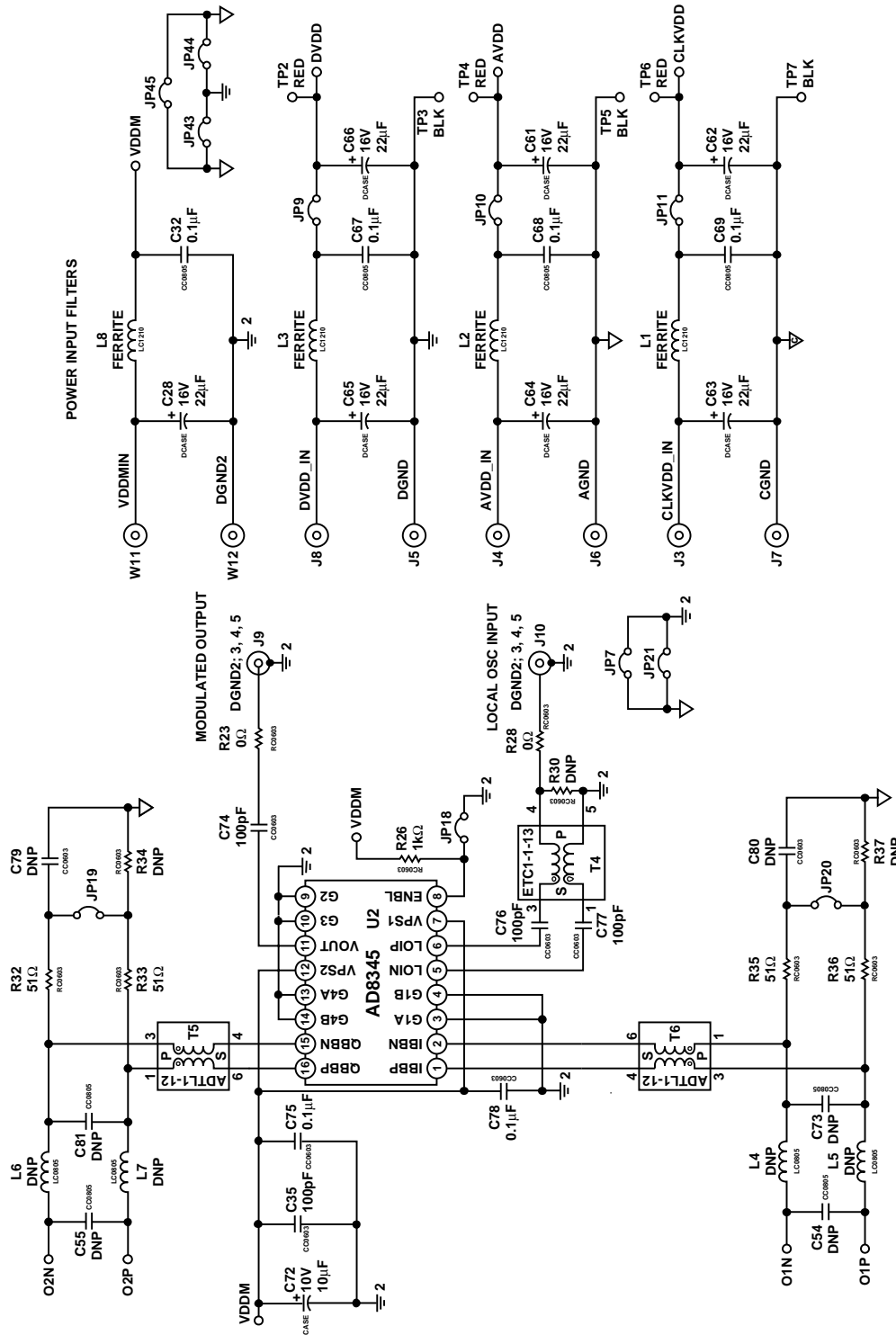
Figure 105. AD8345 Circuitry on AD9777 Evaluation Board
