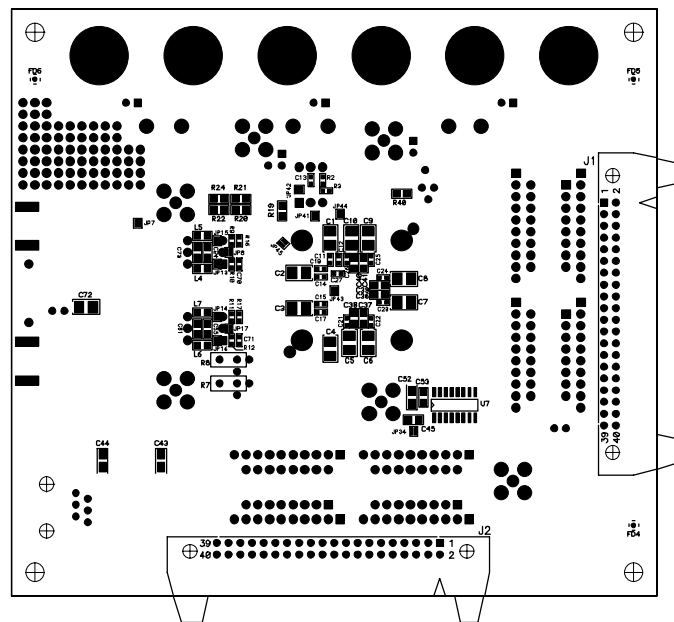
Figure 110. AD9777 Evaluation Board Components, Bottom Side
