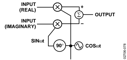
Figure 78. Quadrature Modulation
