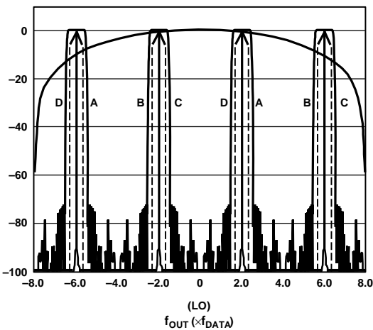
Figure 85. 8x Interpolation, Complex f_{DAC}/4 Modulation
