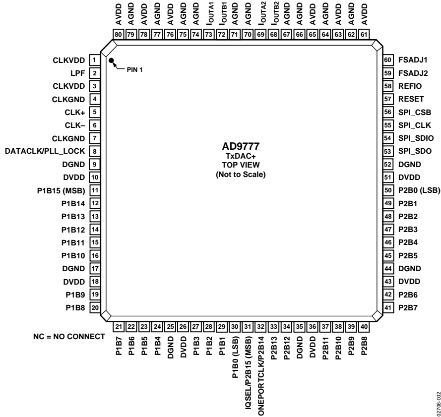
Figure 5. Pin Configuration
