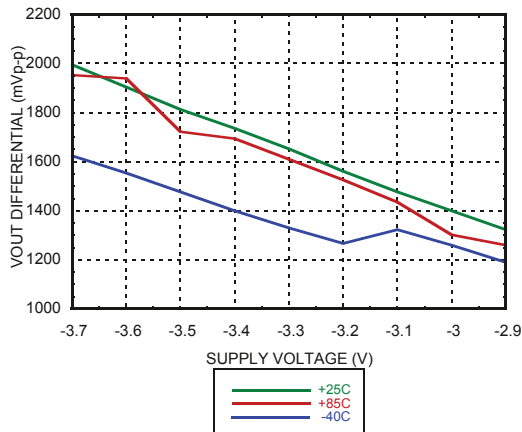
Output Differential Voltage vs. Supply Voltage [1][2]
