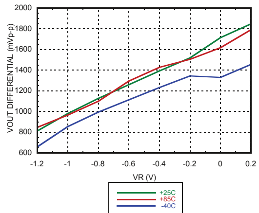
Output Differential Voltage vs. VR [2][3]
