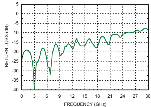
Clock Input Return Loss [1][2][3][4]
