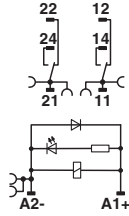
DC coils
