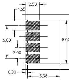
RECOMMENDED PCB LAYOUT TOLERANCE: +/- 0.05
