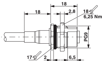
Dimensioned drawing
