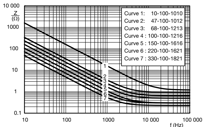
Fig. 10 - Typical impedance as a function of frequency
