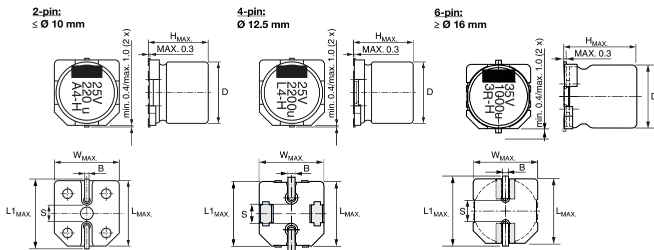
Fig. 2 - Dimensional outline
