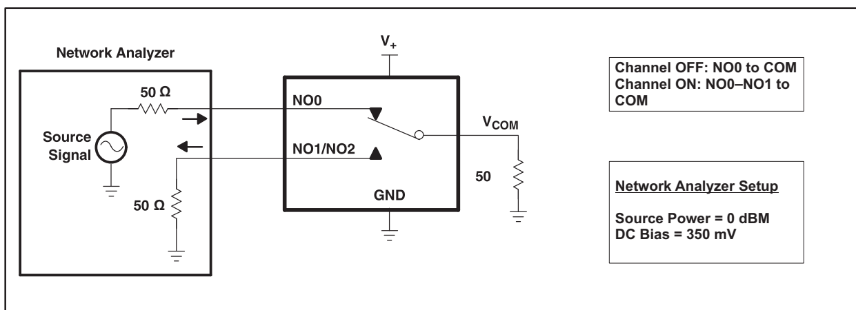
Figure 20. Crosstalk ( X_{TALK} )
