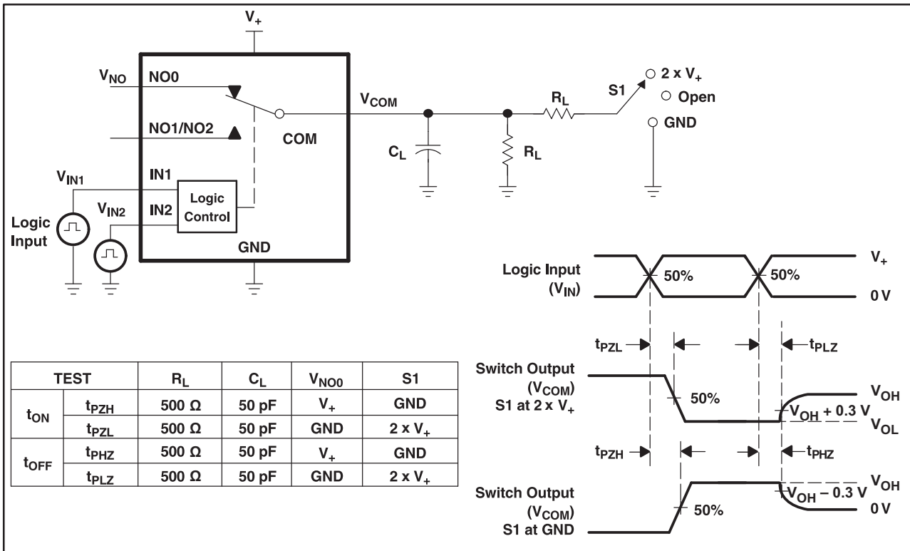
Figure 16. Turn-On ( t_{ON} ) and Turn-Off Time ( t_{OFF} )
