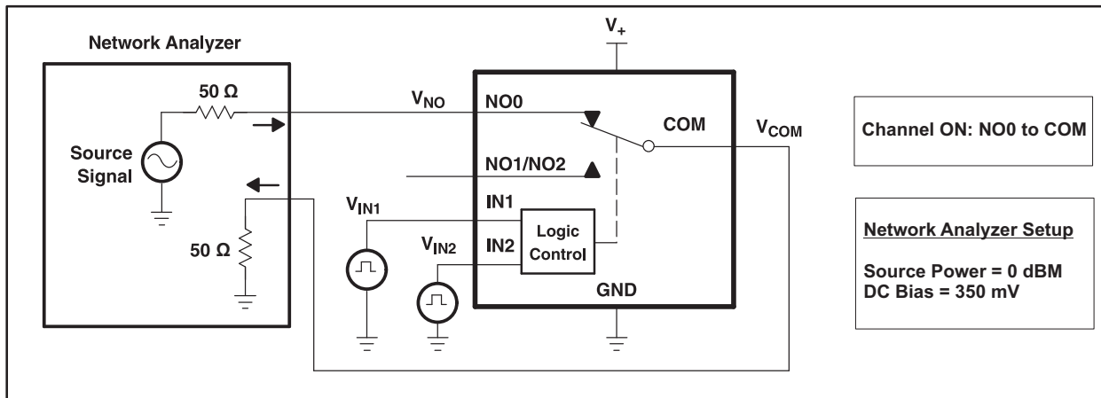
Figure 18. Bandwidth (BW)
