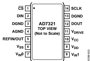
Figure 3. Pin Configuration
