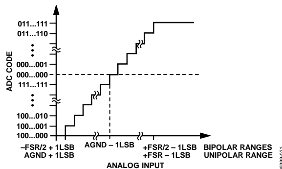
Figure 27. Twos Complement Transfer Characteristic
