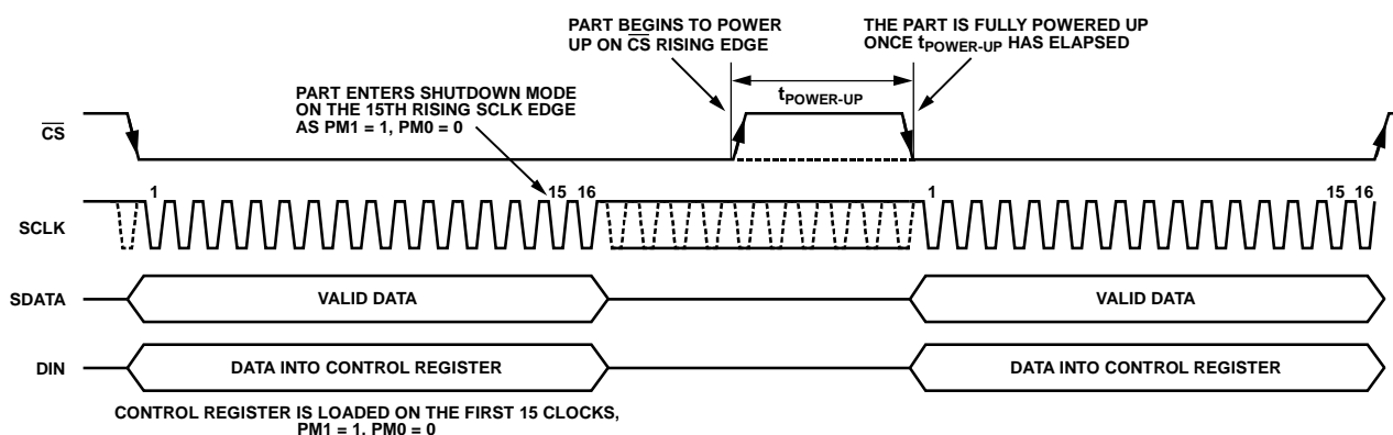
Figure 47. Entering Autoshtutdown/Autostandby Mode
