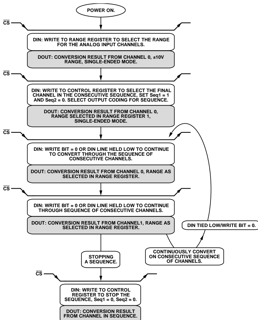
Figure 44. Flowchart for Consecutive Sequence of Channels
