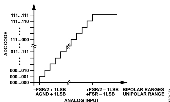
Figure 28. Straight Binary Transfer Characteristic
