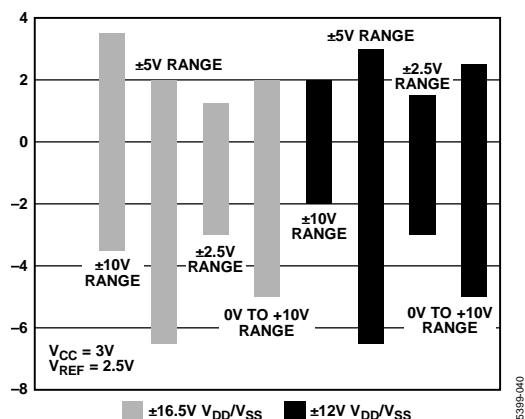
Figure 41. Pseudo Input Range with V_{CC} = 3\text{ V}
