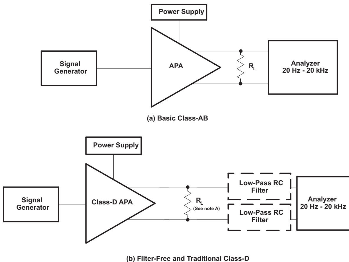
Figure 35. Audio Measurement Systems
