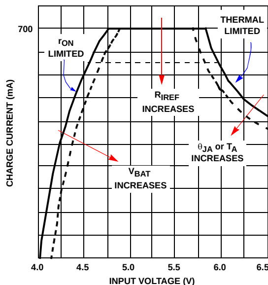
FIGURE 1. CHARGE CURRENT LIMITS IN THE CC MODE
