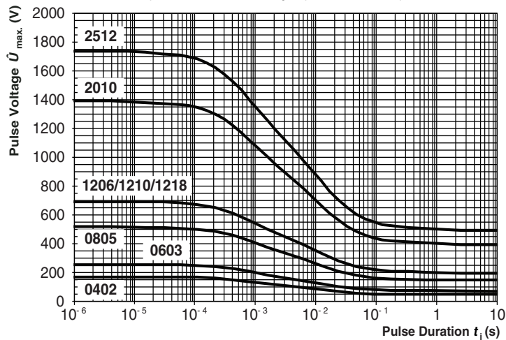
Maximum pulse voltage, single and continuous pulses; applicable if \bar{P} \leq \bar{P}_{max} ; for permissible resistance change equivalent to 8000 h operation
