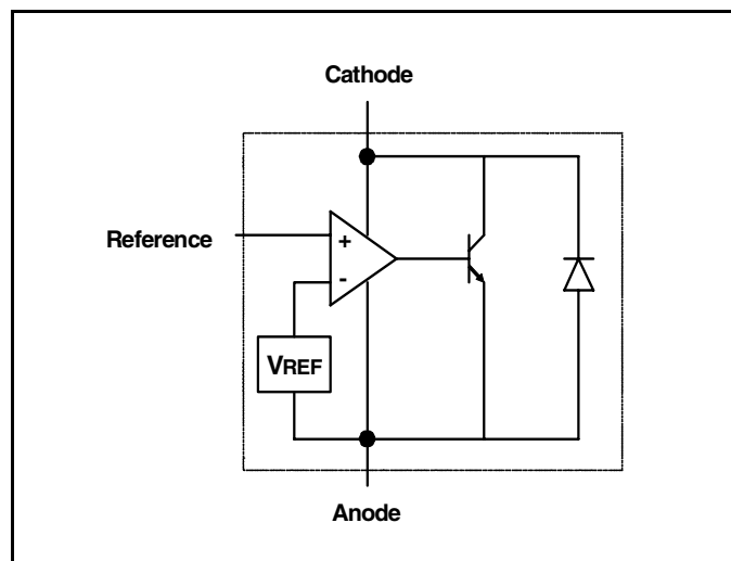
Figure 15. Block diagram
