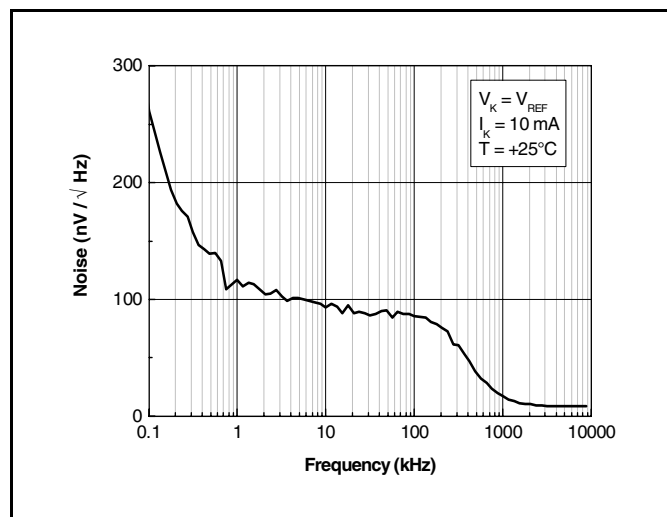
Figure 18. Equivalent input noise vs frequency
