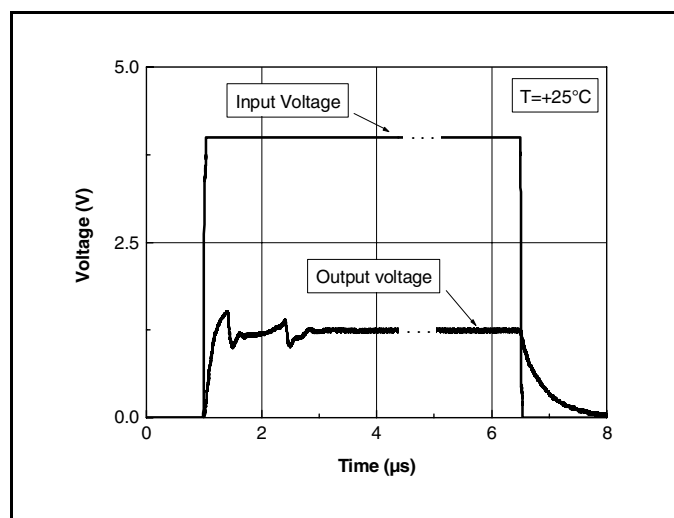
Figure 14. Pulse response at I_K = 10\text{mA}
