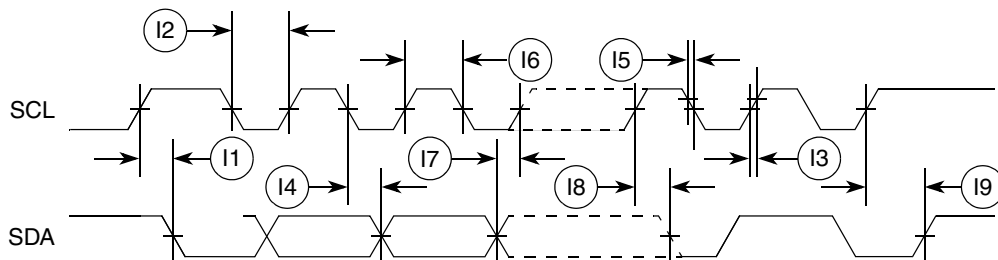
Figure 23. I 2 C Input/Output Timings
