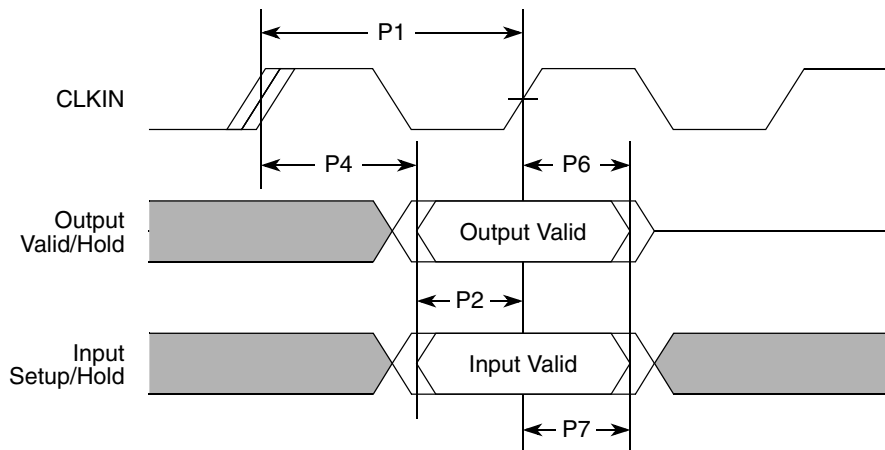
Figure 18. PCI Timing
