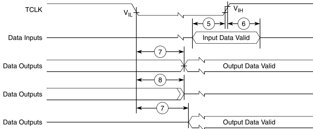
Figure 25. Boundary Scan (JTAG) Timing
