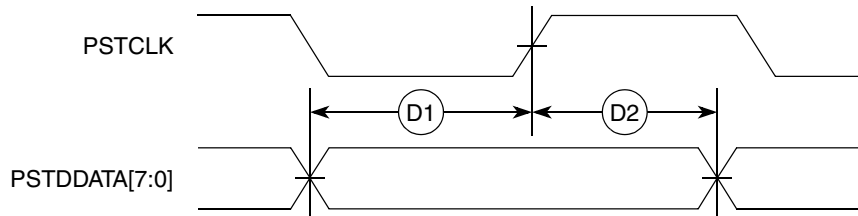
Figure 28. Real-Time Trace AC Timing
