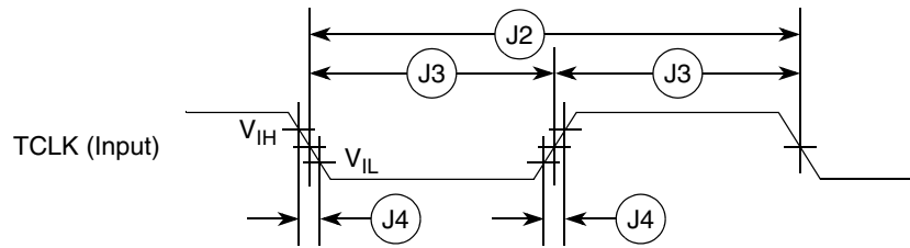
Figure 24. Test Clock Input Timing
