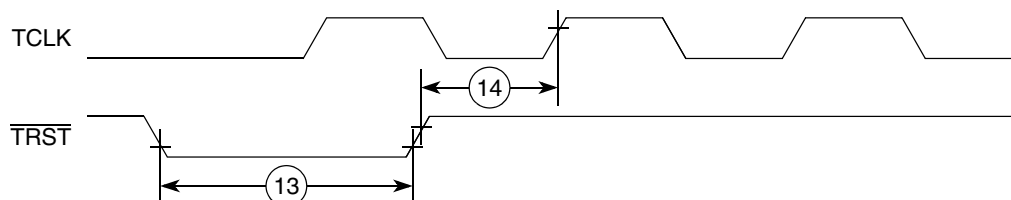
Figure 27. TRST Timing Debug AC Timing Specifications
