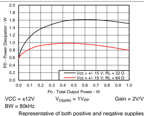
Figure 8. Power Dissipation versus Total Output Power
