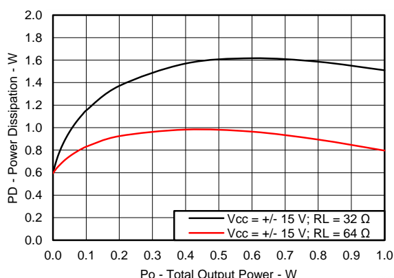
Figure 18. Power Dissipation versus Output Power
