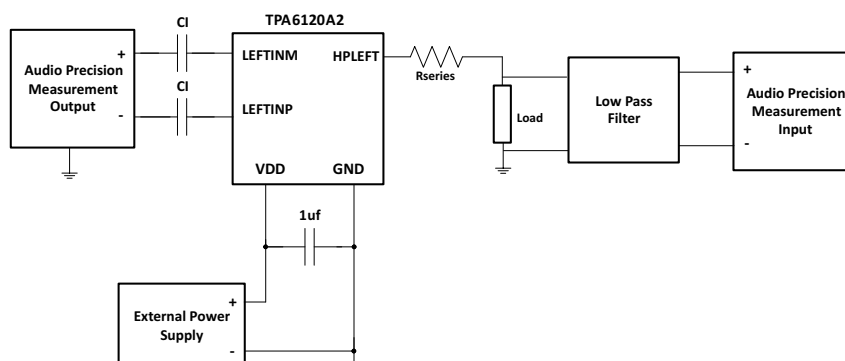
Figure 12. Test Circuit
