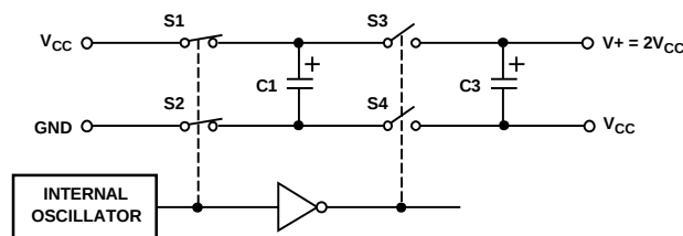
Figure 29. Charge Pump Voltage Doubler
