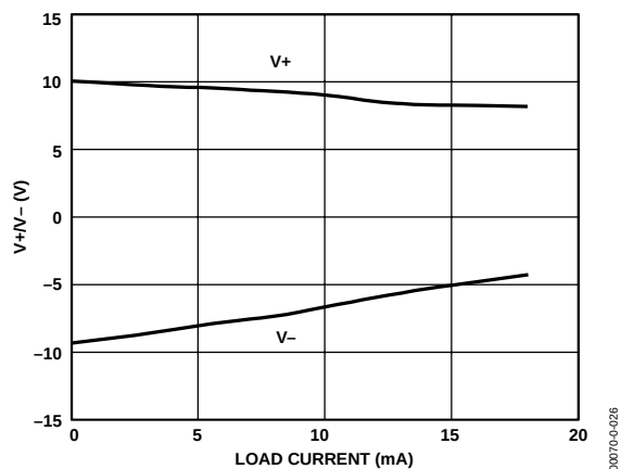
Figure 12. Charge Pump V+ and V- vs. Current
