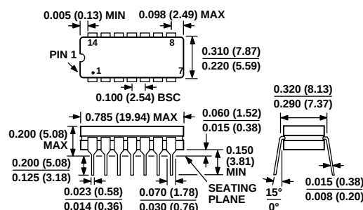
Figure 35. 14-Lead Ceramic Dual In-Line Package [CERDIP] (Q-14)
