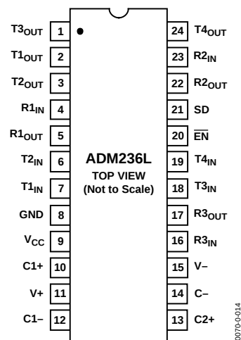
Figure 7. ADM236L PDIP/SOIC Pin Configuration
