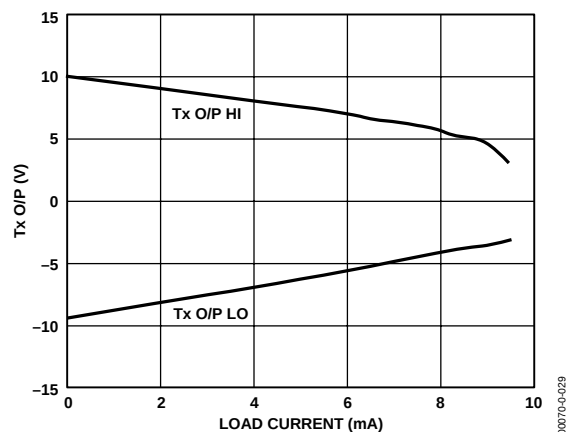
Figure 15. Transmitter Output Voltage vs. Current
