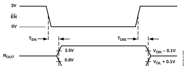
Figure 31. Enable Timing
