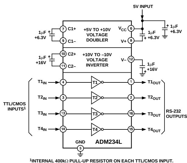
Figure 20. ADM234L Typical Operating Circuit
