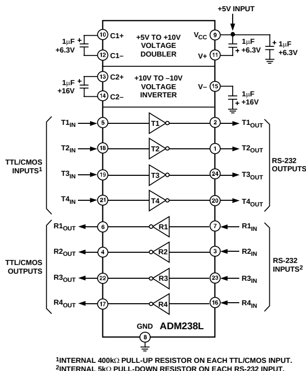
Figure 23. ADM238L Typical Operating Circuit
