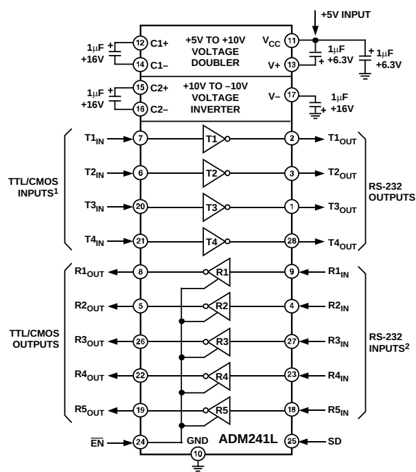
Figure 25. ADM241L Typical Operating Circuit
