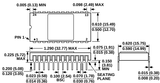
Figure 41. 24-Lead Side-Braced Ceramic Dual In-Line Package [SBDIP] (D-24-2) Dimensions shown in inches and (millimeters)
