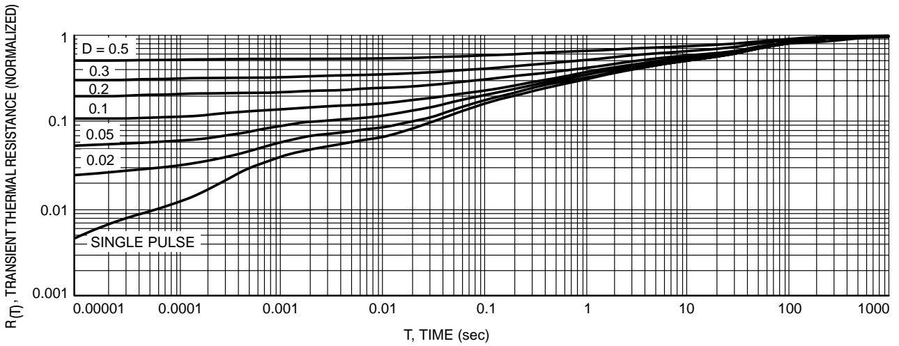
Figure 7. Thermal Resistance
