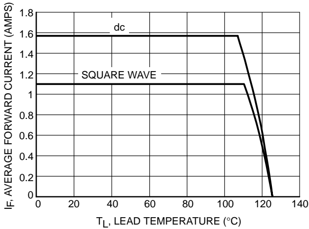
Figure 5. Current Derating - Lead
