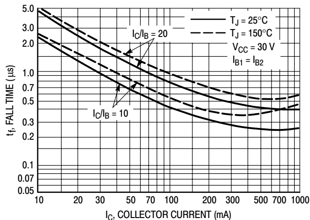
Figure 7. Fall Time
