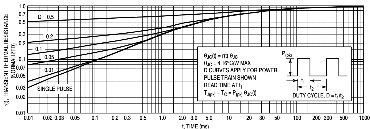
Figure 4. Thermal Response
