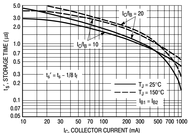
Figure 6. Storage Time
