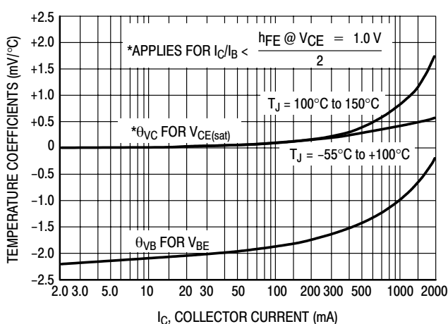
Figure 13. Temperature Coefficients
