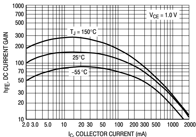
Figure 8. Current Gain
