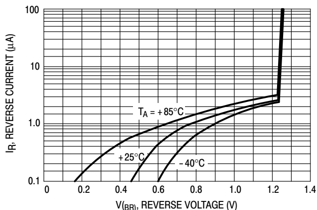
Figure 2. Reverse Characteristics
