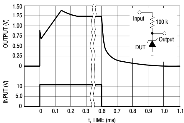
Figure 7. Response Time
