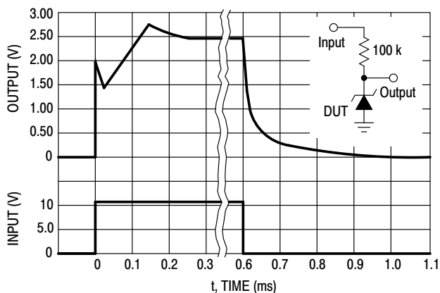
Figure 13. Response Time
