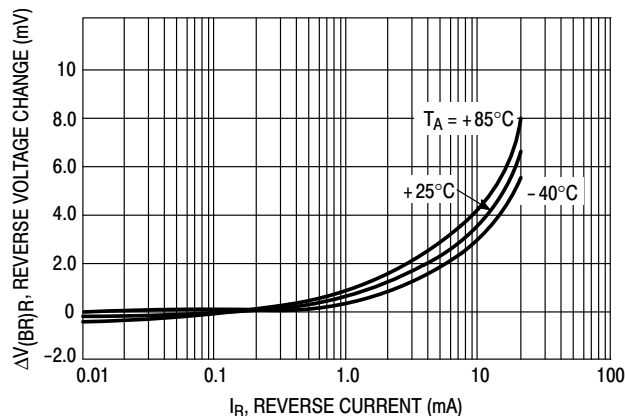
Figure 9. Reverse Characteristics
