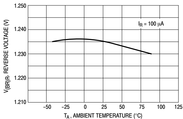
Figure 5. Temperature Drift
