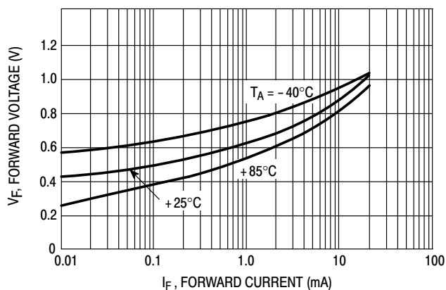
Figure 10. Forward Characteristics
