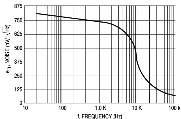
Figure 6. Noise Voltage
