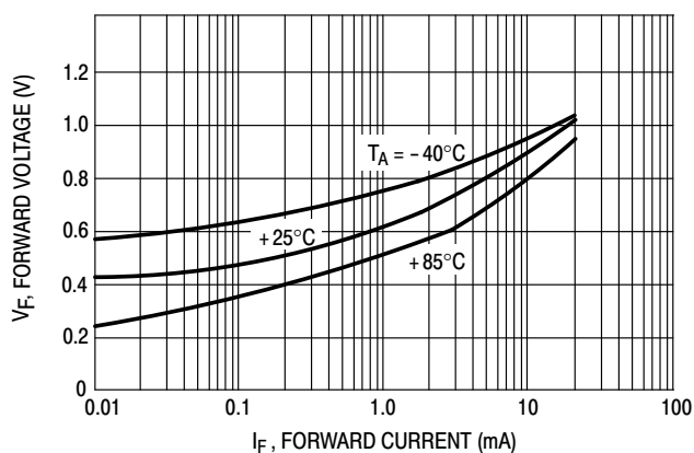
Figure 4. Forward Characteristics
