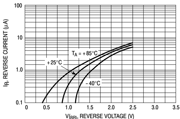
Figure 8. Reverse Characteristics
