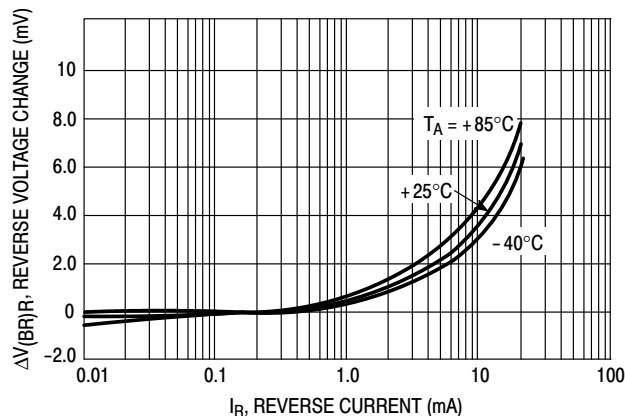
Figure 3. Reverse Characteristics
