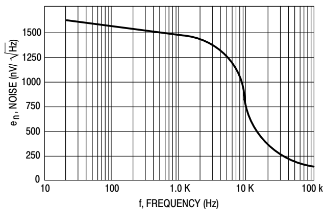
Figure 12. Noise Voltage
