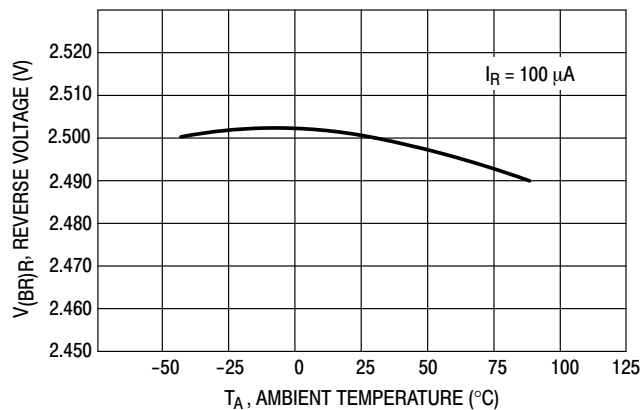
Figure 11. Temperature Drift
