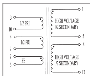
Schematic E
