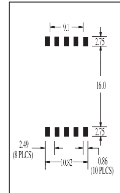
Pad Layout B
