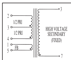
Schematic A
