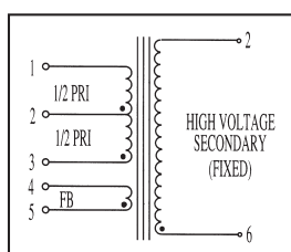
Schematic D
