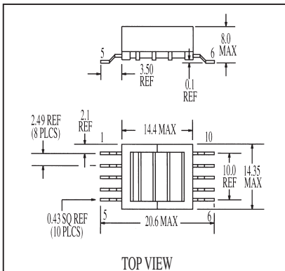
Schematic A
