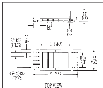
Mechanical C
