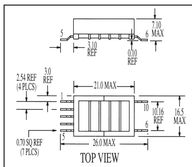
Mechanical F
