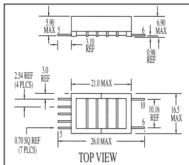
Mechanical E
