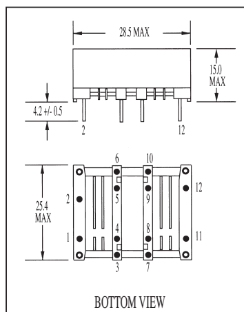
Mechanical G
