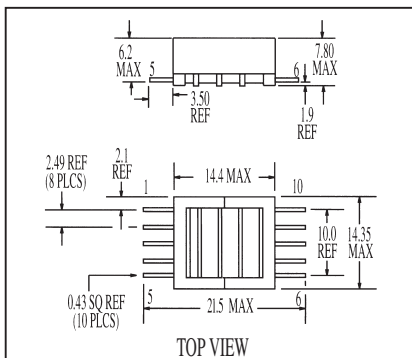
Mechanical A
