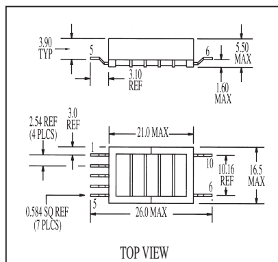
Mechanical D
