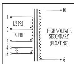
Schematic C
