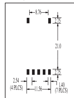
Pad Layout C
