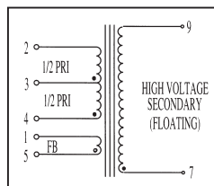
Schematic B
