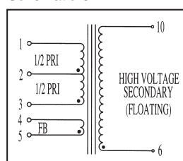
Schematic C
