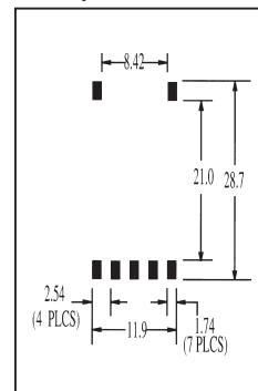
Pad Layout C
