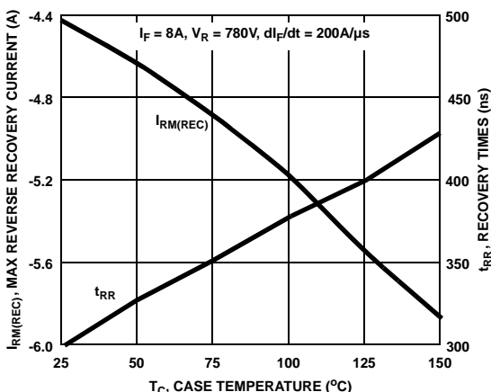
Figure 10. Reverse Recovery Current and Times vs Case Temperature
