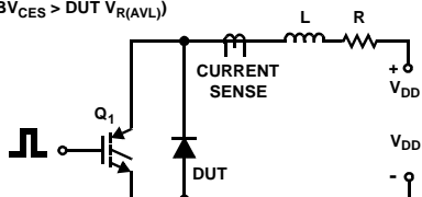
Figure 15. Avalanche Energy Test Circuit
