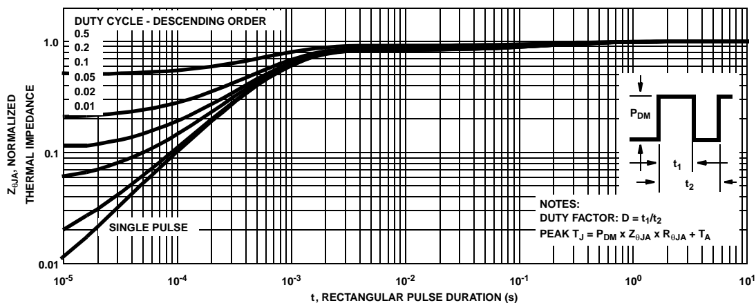
Figure 12. Normalized Maximum Transient Thermal Impedance
