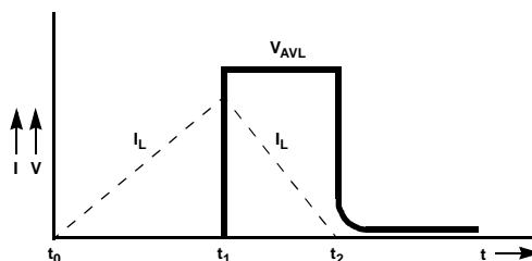
Figure 16. Avalanche Current and Voltage Waveforms
