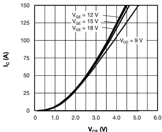
Fig. 2 - Typical IGBT Output Characteristics, T_J = 125\text{ °C}
