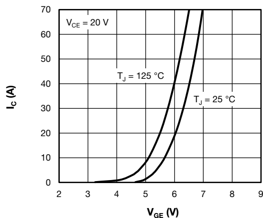
Fig. 5 - Typical IGBT Transfer Characteristics
