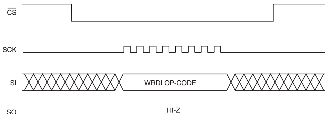
Figure 5. WRDI Timing
