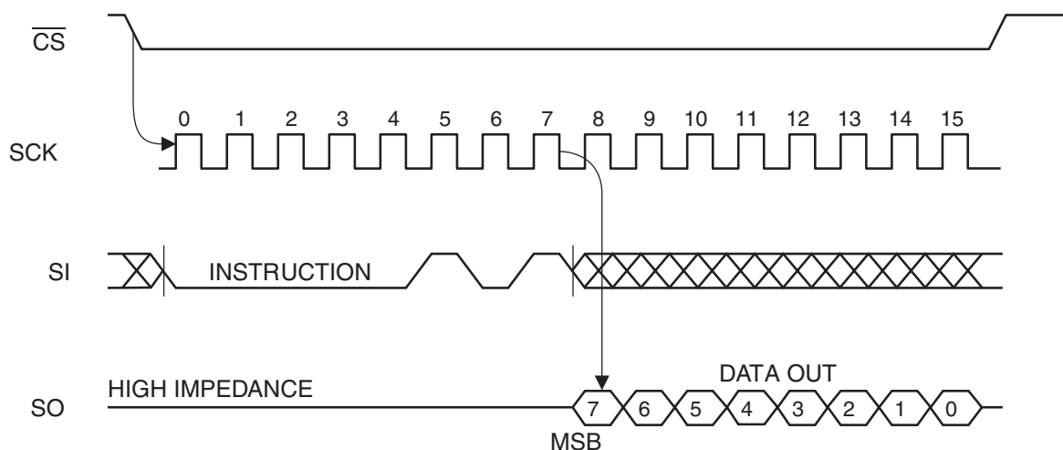
Figure 6. RDSR Timing
