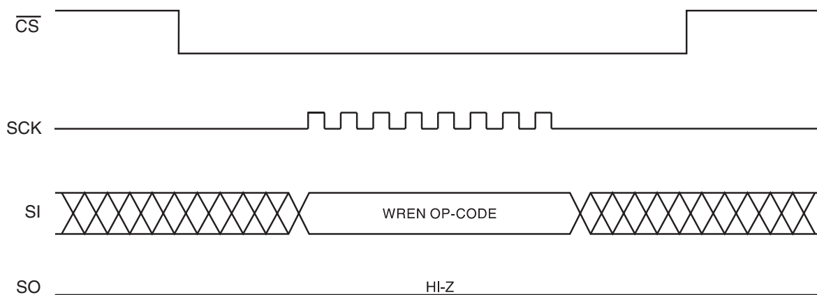
Figure 4. WREN Timing
