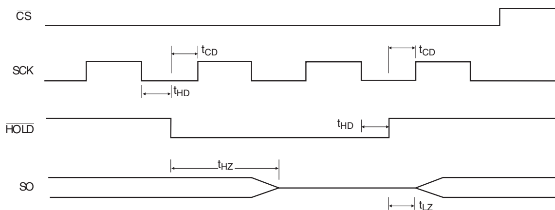
Figure 11. HOLD Timing
