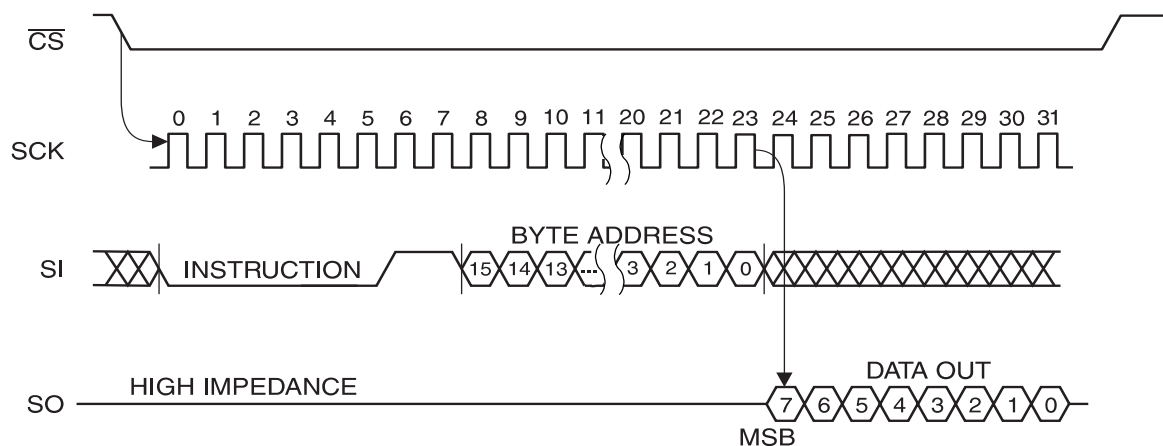
Figure 8. READ Timing
