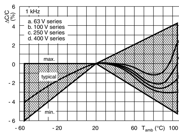
Capacitance as a function of ambient temperature
