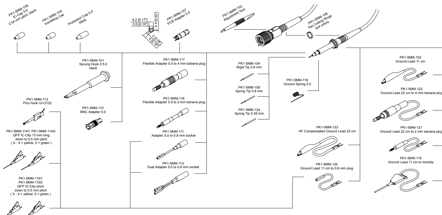
Probe Accessory Diagram for PP005A, PP009 and PP011 Passive Probes
