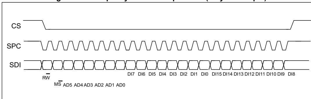
Figure 10. Multiple byte SPI write protocol (2-byte example)
