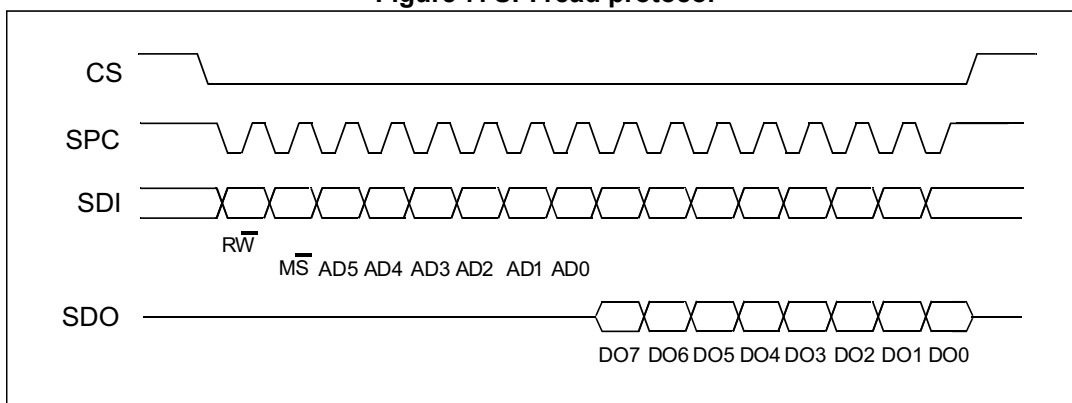
Figure 7. SPI read protocol
