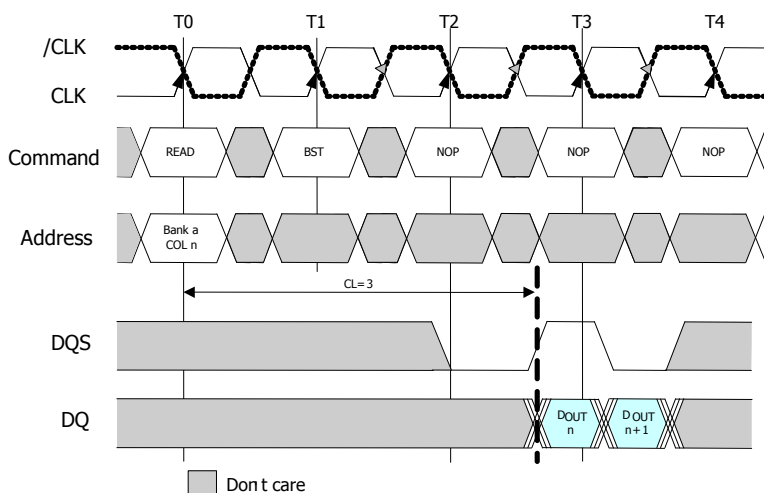
Figure17 : Read Burst terminate (BL=4,8 or 16)
