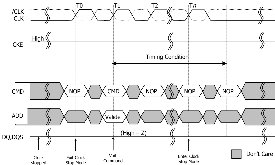
Figure 37 : Clock Stop Mode
