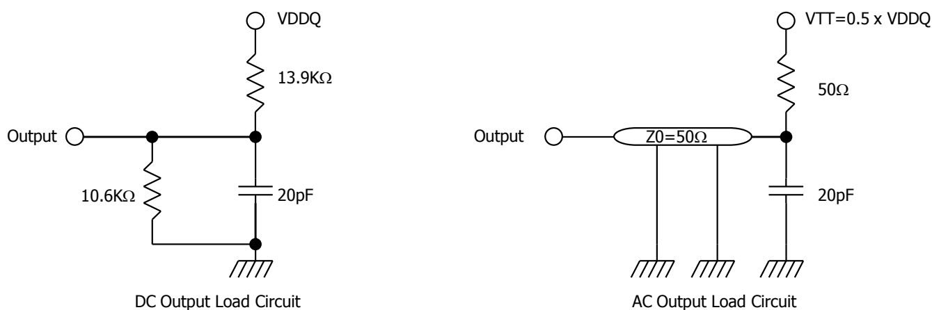
Figure8: Output load circuit
