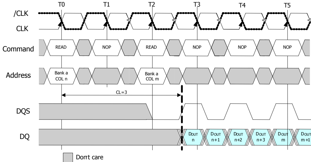
Figure14 : Consecutive Read bursts (BL=4)
