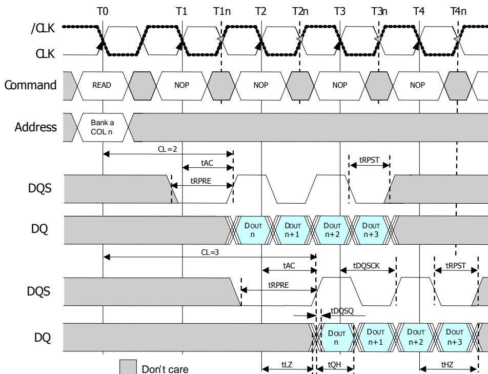
Figure13 : Read Data out timing (BL=4)
