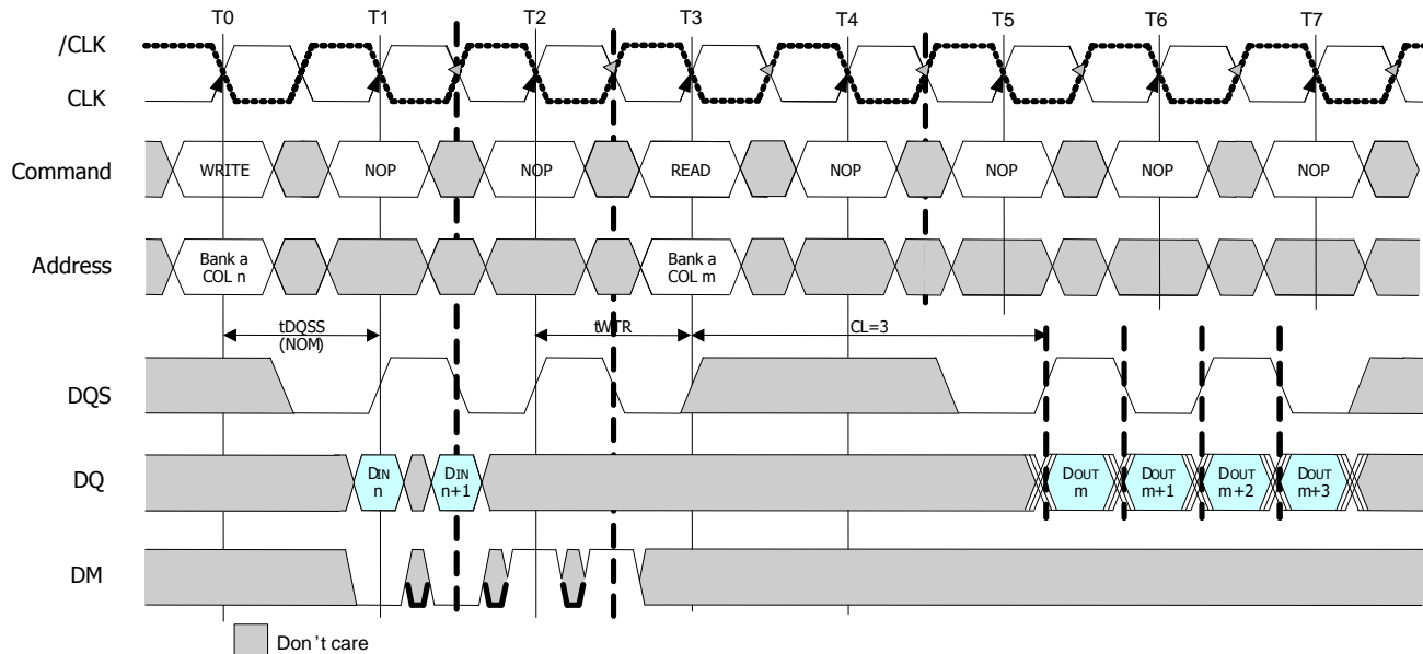
Figure26 : Write to Read (Interrupting)
