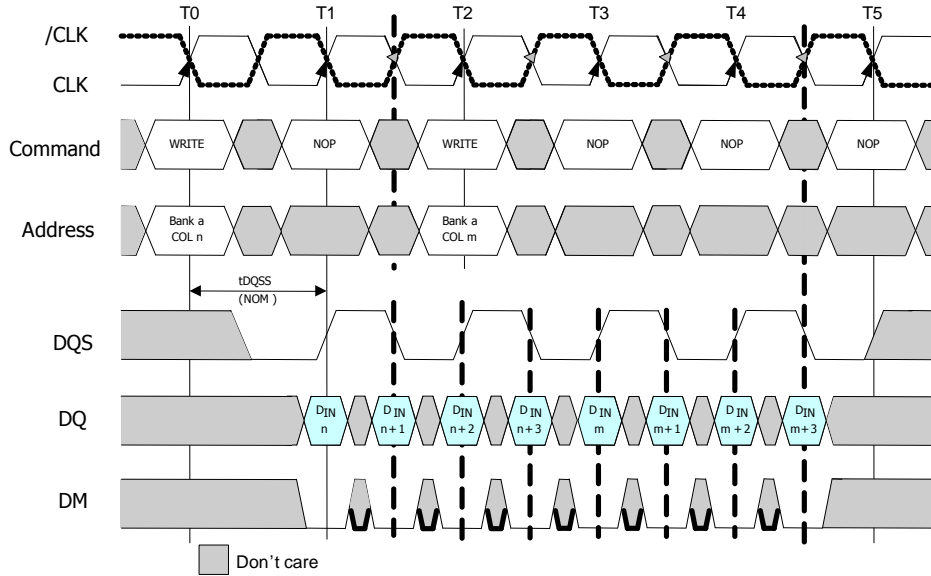
Figure22 : Consecutive Write to write (BL=4)
