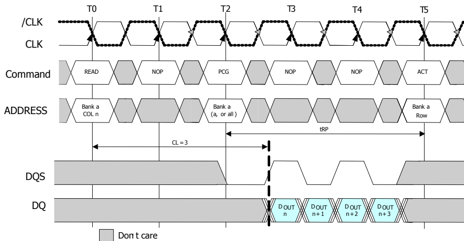
Figure19 : Read to Precharge (BL=4)
