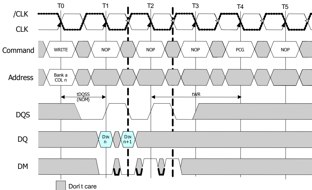
Figure29 : Write to Precharge (Interrupting)
