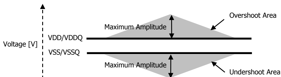
Figure9: AC Overshoot/Undershoot Definition
