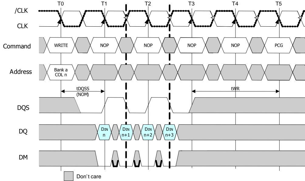
Figure28 : Write to Precharge (Uninterrupting)
