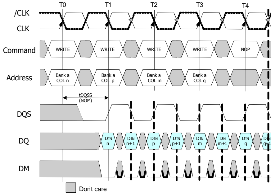
Figure24 : Random Write to write
