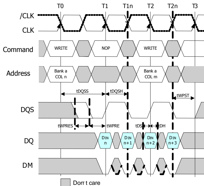
Figure21 : Write Burst (BL=4)
