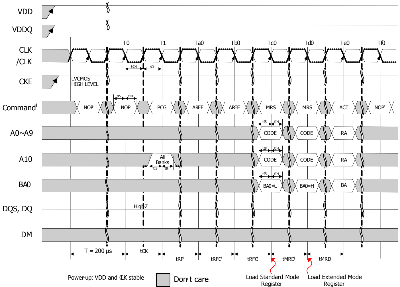
Figure6 : Power up sequence
