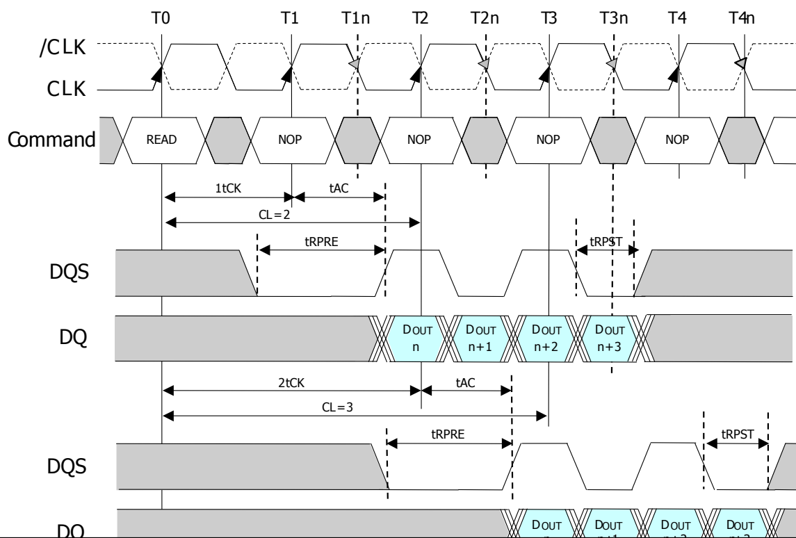
Figure7 : CAS Latency (BL=4)
