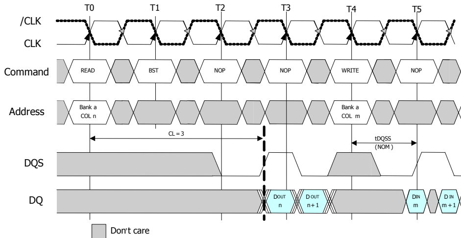
Figure18 : Read to write terminate (BL=4,8 or 16)
