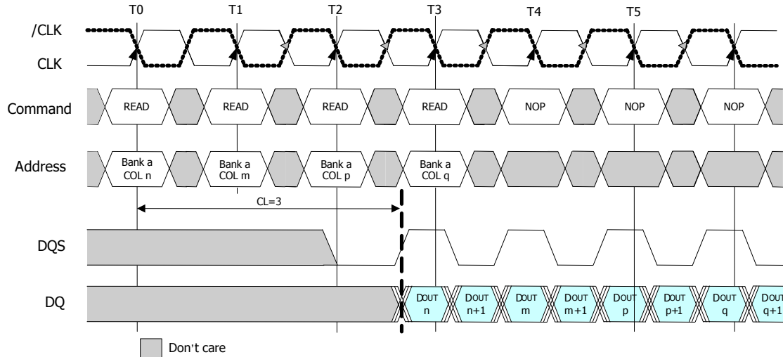
Figure16 : Random Read access
