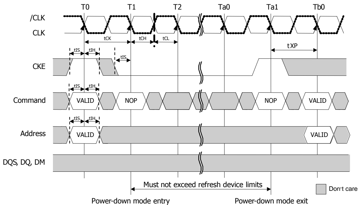
Figure35 : Power down (Active or Precharge)
