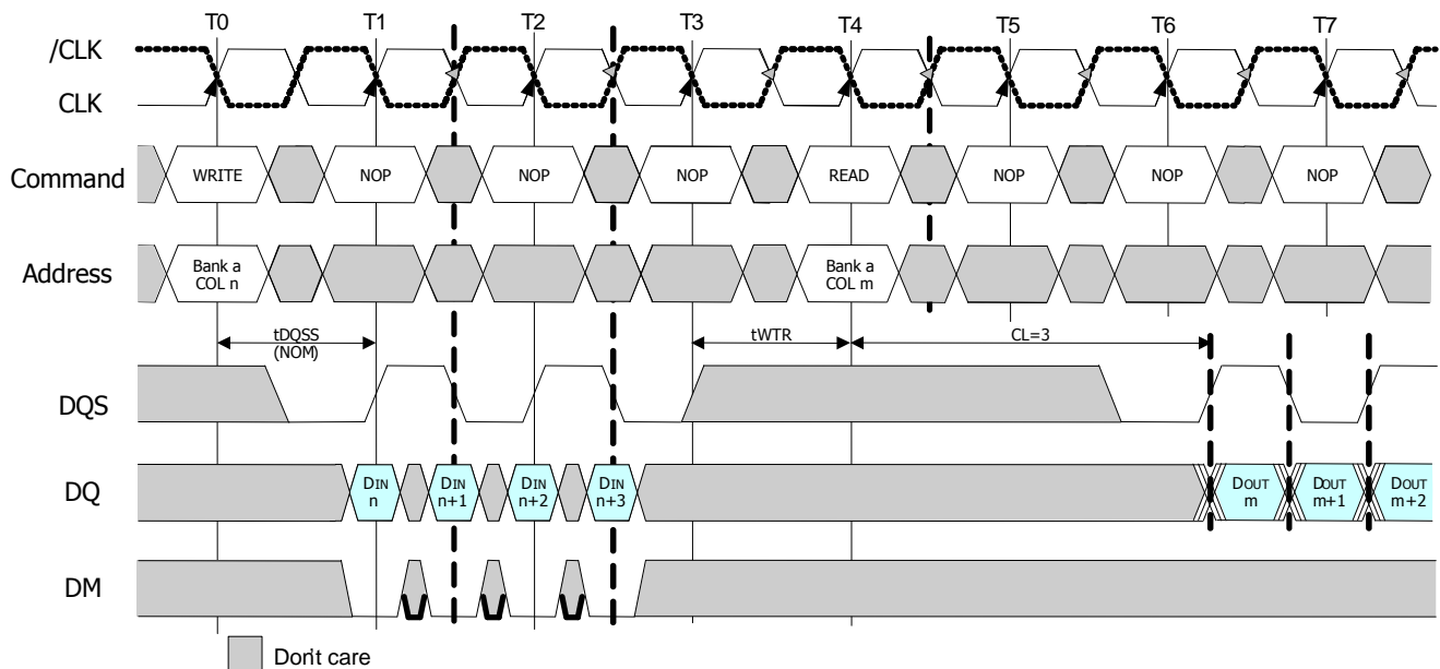
Figure25 : Write to Read (Uninterrupting)
