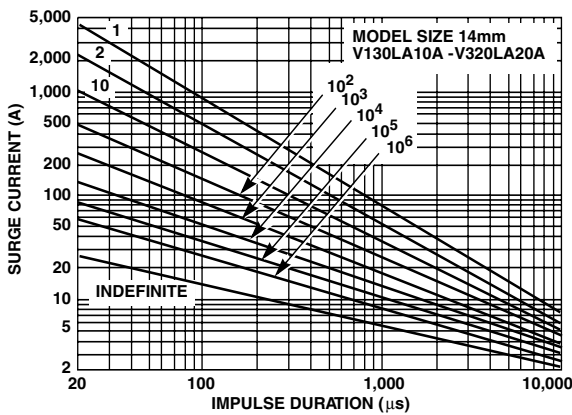
FIGURE 16. SURGE CURRENT RATING CURVES FOR V130LA10A - V320LA20A
