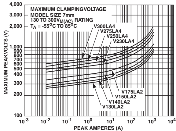
FIGURE 4. CLAMPING VOLTAGE FOR V130LA2 - V300LA4
