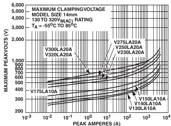
FIGURE 8. CLAMPING VOLTAGE FOR V130LA10A - V320LA20A
