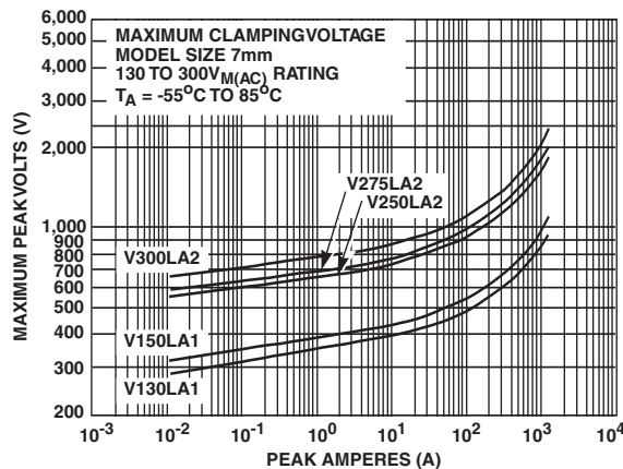
FIGURE 3. CLAMPING VOLTAGE FOR V130LA1 - V300LA2
