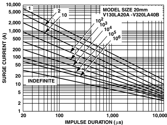
FIGURE 18. SURGE CURRENT RATING CURVES FOR V130LA20A - V320LA40B
