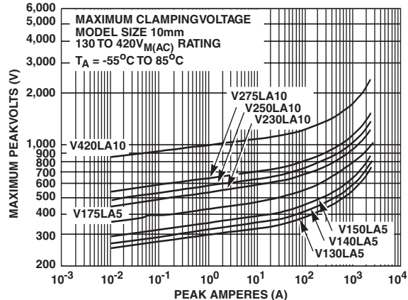
FIGURE 6. CLAMPING VOLTAGE FOR V130LA5 - V420LA10
