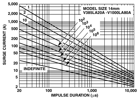
FIGURE 17. SURGE CURRENT RATING CURVES FOR V385LA20A - V1000LA80A
