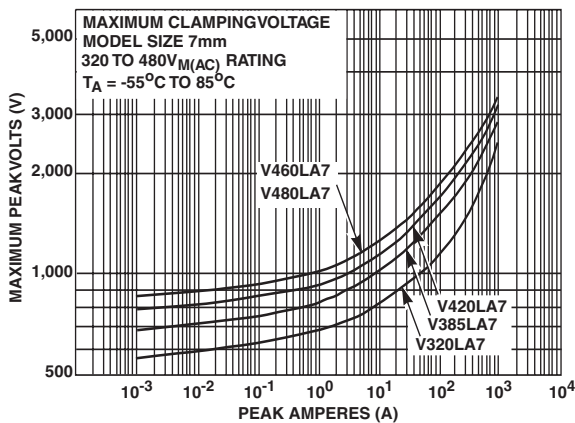
FIGURE 5. CLAMPING VOLTAGE FOR V320LA7 - V480LA7
