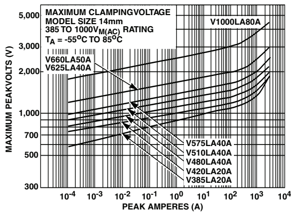
FIGURE 9. CLAMPING VOLTAGE FOR V385LA20A - V1000LA80A
