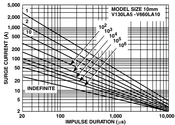
FIGURE 15. SURGE CURRENT RATING CURVES FOR V130LA5 - V660LA10
