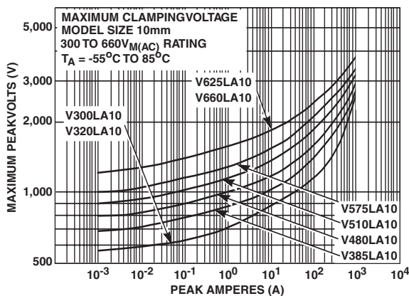
FIGURE 7. CLAMPING VOLTAGE FOR V300LA10 - V660LA10
