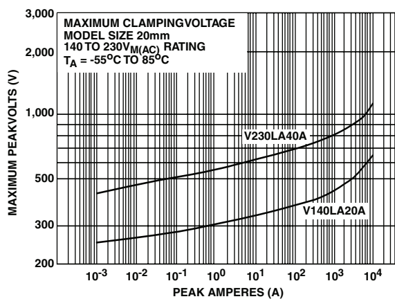
FIGURE 12. CLAMPING VOLTAGE FOR V140LA20A - V230LA40A
