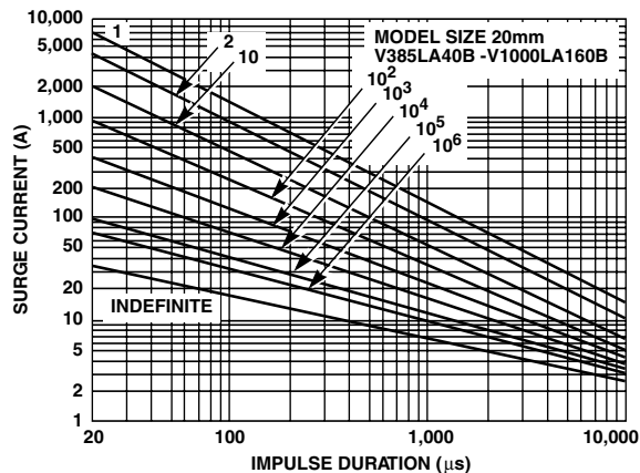
FIGURE 19. SURGE CURRENT RATING CURVES FOR V385LA40B - V1000LA160B
