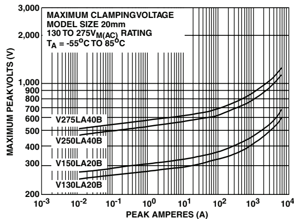
FIGURE 11. CLAMPING VOLTAGE FOR V130LA20B - V275LA40B
