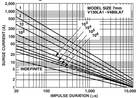
FIGURE 14. SURGE CURRENT RATING CURVES FOR V130LA1 - V480LA7
