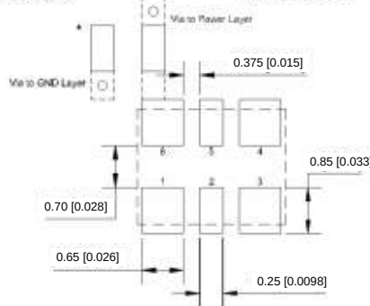
Recommended Solder Pad Layout units: mm[inch]
