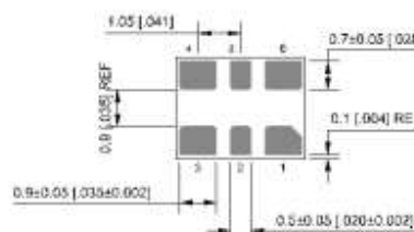
External Dimensions units: mm[inch]
