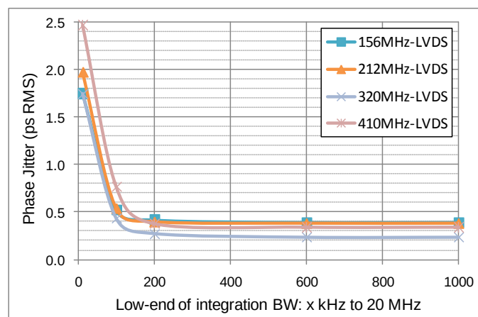
Phase jitter (integrated phase noise)
