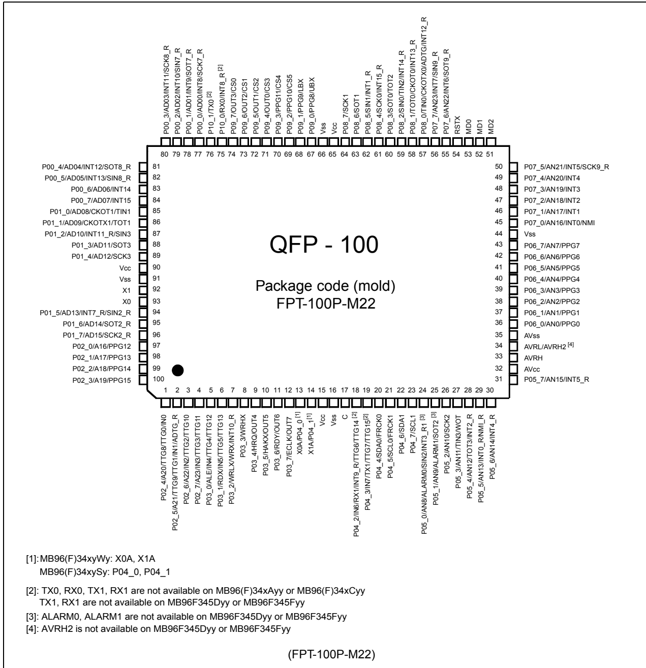
Figure 2. Pin assignment of MB96(F)34x (FPT-100P-M22)
