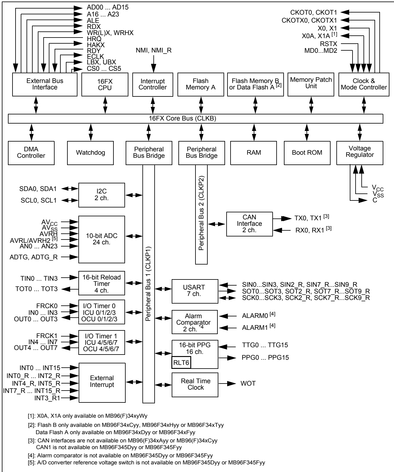
Figure 1. Block diagram of MB96(F)34x
