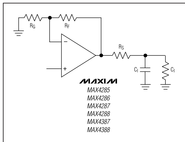
Figure 1. Using an Isolation Resistor ( R_S ) for High Capacitive Loads
