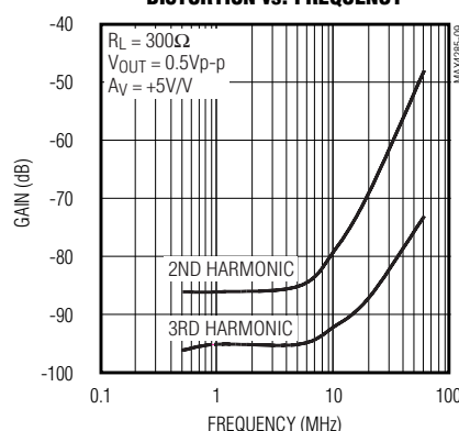
MAX4286/MAX4387/MAX4388 DISTORTION vs. FREQUENCY
