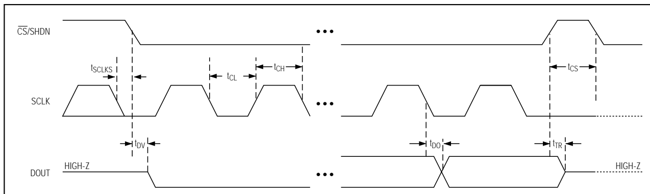
Figure 7. Detailed Serial-Interface Timing Sequence
