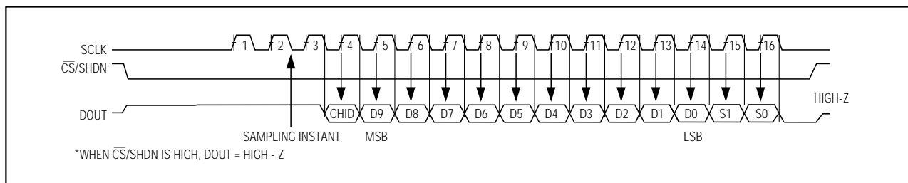
Figure 9b. QSPI Interface Timing Sequence (CPOL = CPHA = 0)
