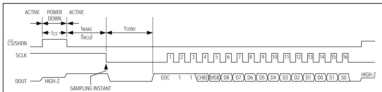
Figure 5. Internal Clock Mode Timing
