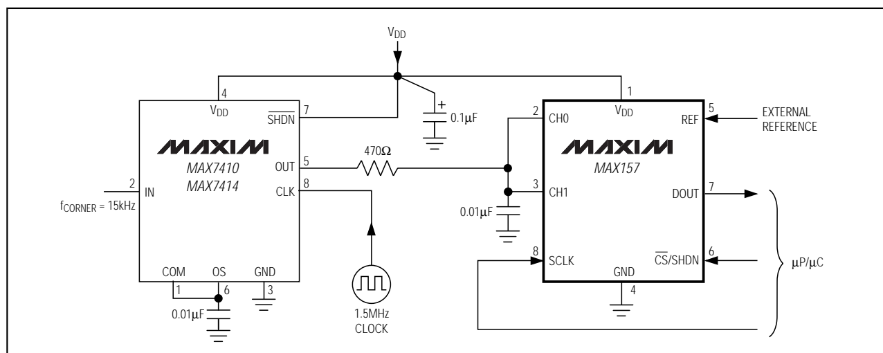
Figure 4. Analog Input with Anti-Aliasing Filter Structure
