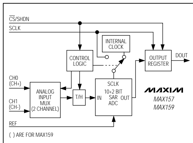
Figure 2. MAX157/MAX159 Simplified Functional Diagram
