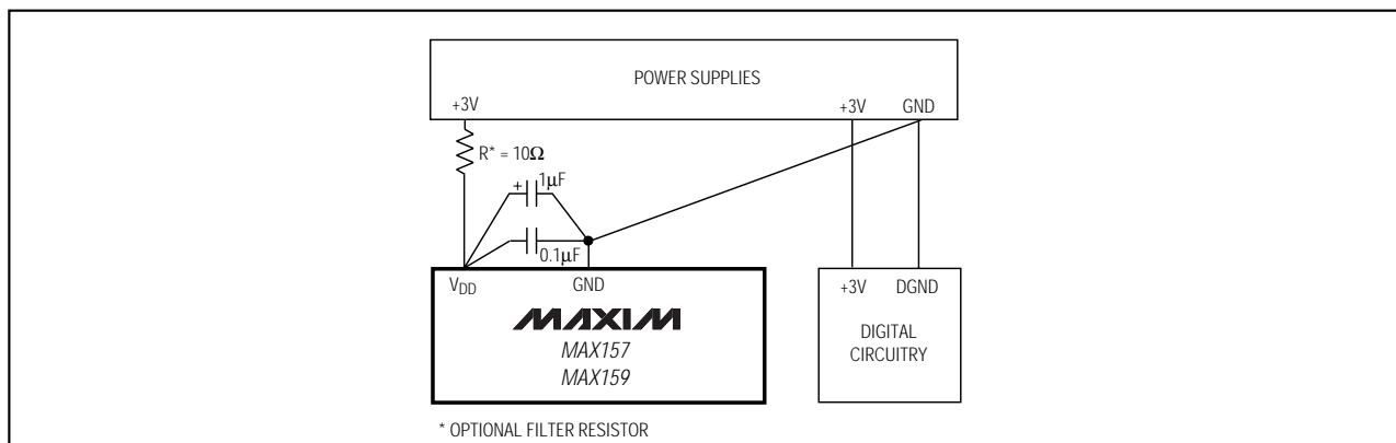
Figure 11. Power-Supply Bypassing and Grounding
