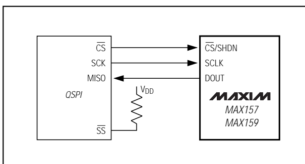
Figure 9a. QSPI Connections
