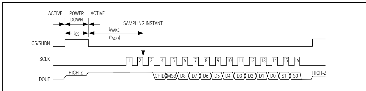
Figure 6. External Clock Mode Timing
