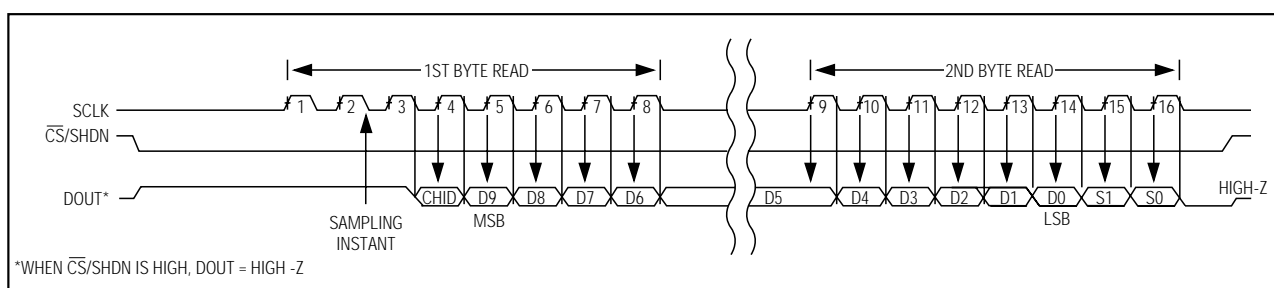
Figure 8c. SPI/MICROWIRE Interface Timing Sequence (CPOL = CPHA = 0)
