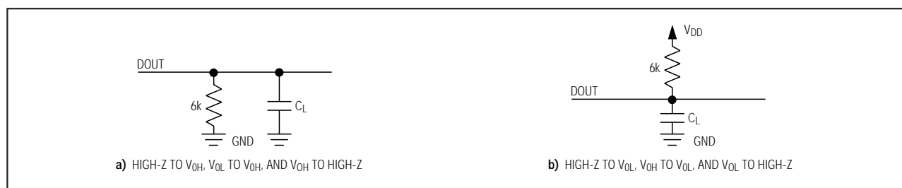
Figure 1. Load Circuits for Enable and Disable Time
