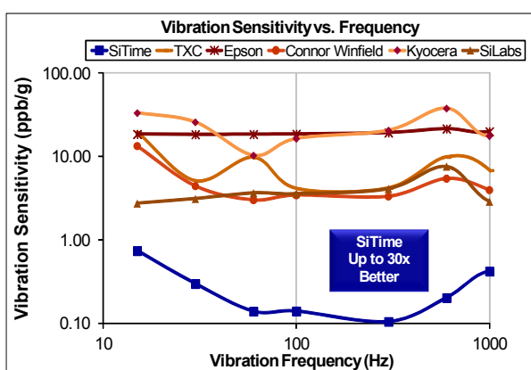
Figure 5. Vibration Robustness [5]
