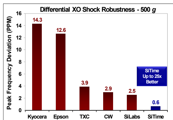
Figure 6. Shock Robustness [6]
