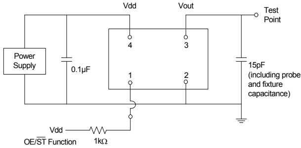
Figure 1. Test Circuit
