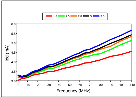
Figure 7. Idd vs Frequency
