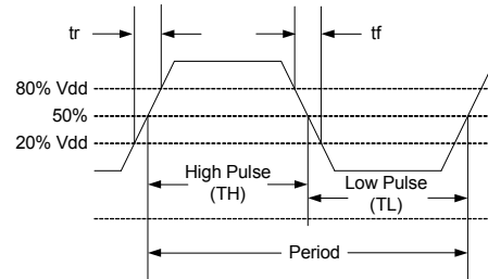
Figure 2. Waveform
