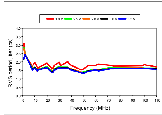
Figure 8. RMS Period Jitter vs Frequency
