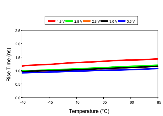
Figure 12. Rise Time vs Temperature, 20 MHz Output
