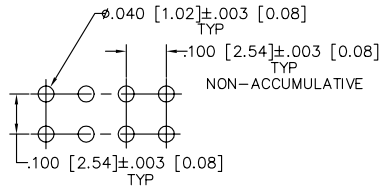
RECOMMENDED HOLE PATTERN
