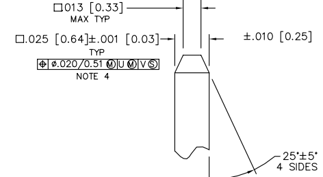
DETAIL P SCALE 5:1 TYP BOTH ENDS
