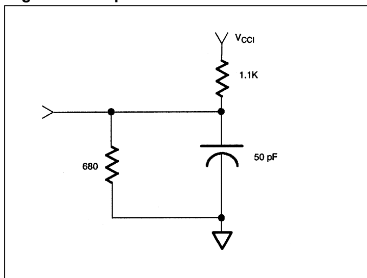
Figure 15. Output Load
