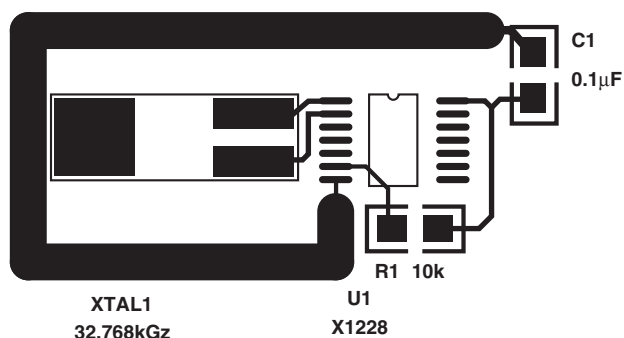
Figure 15. Suggested Layout for Intersil RTC in SO-14
