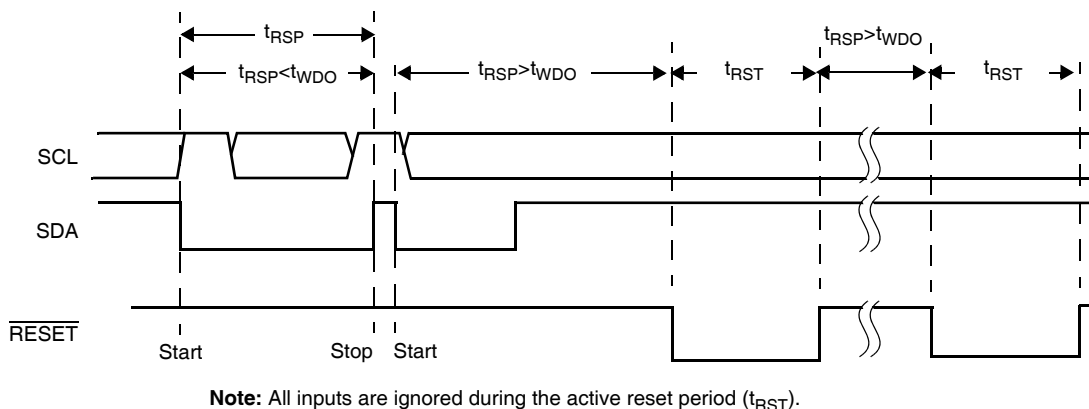
Figure 3. Watchdog Restart/Time Out
