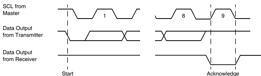
Figure 9. Acknowledge Response From Receiver
