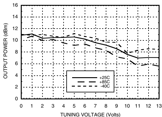
vs. Tuning Voltage, V_{cc} = +5V
