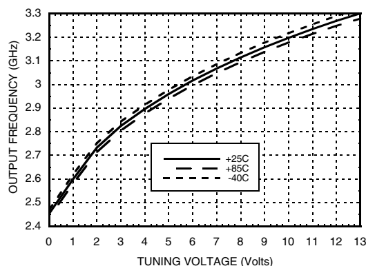
Divide-by-4 Frequency vs. Tuning Voltage, V_{cc} = +5V
