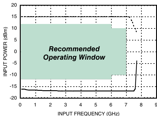
Input Sensitivity Window, T = 25^\circ\text{C}
