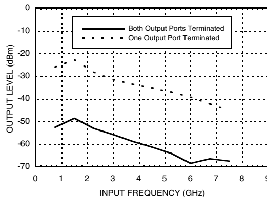
Reverse Leakage, P_{in} = 0\text{ dBm} , T = 25^\circ\text{C}
