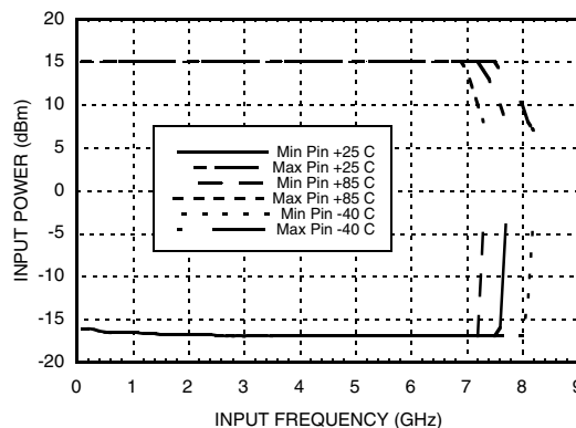
Input Sensitivity Window vs. Temperature
