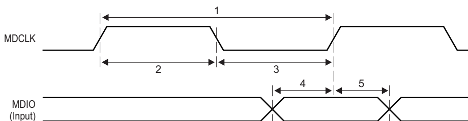
Figure 10-49 MDIO Input Timing
