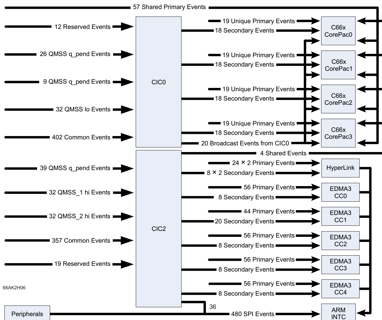
Figure 6-5 66AK2H06 Interrupt Topology
