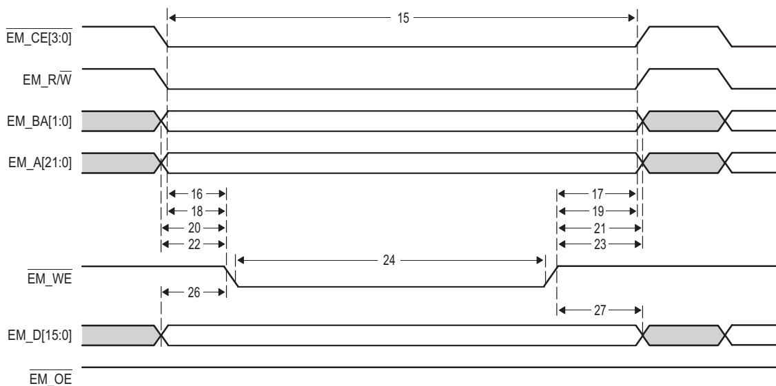
Figure 10-55 EMIF16 EM_WAIT Read Timing Diagram
