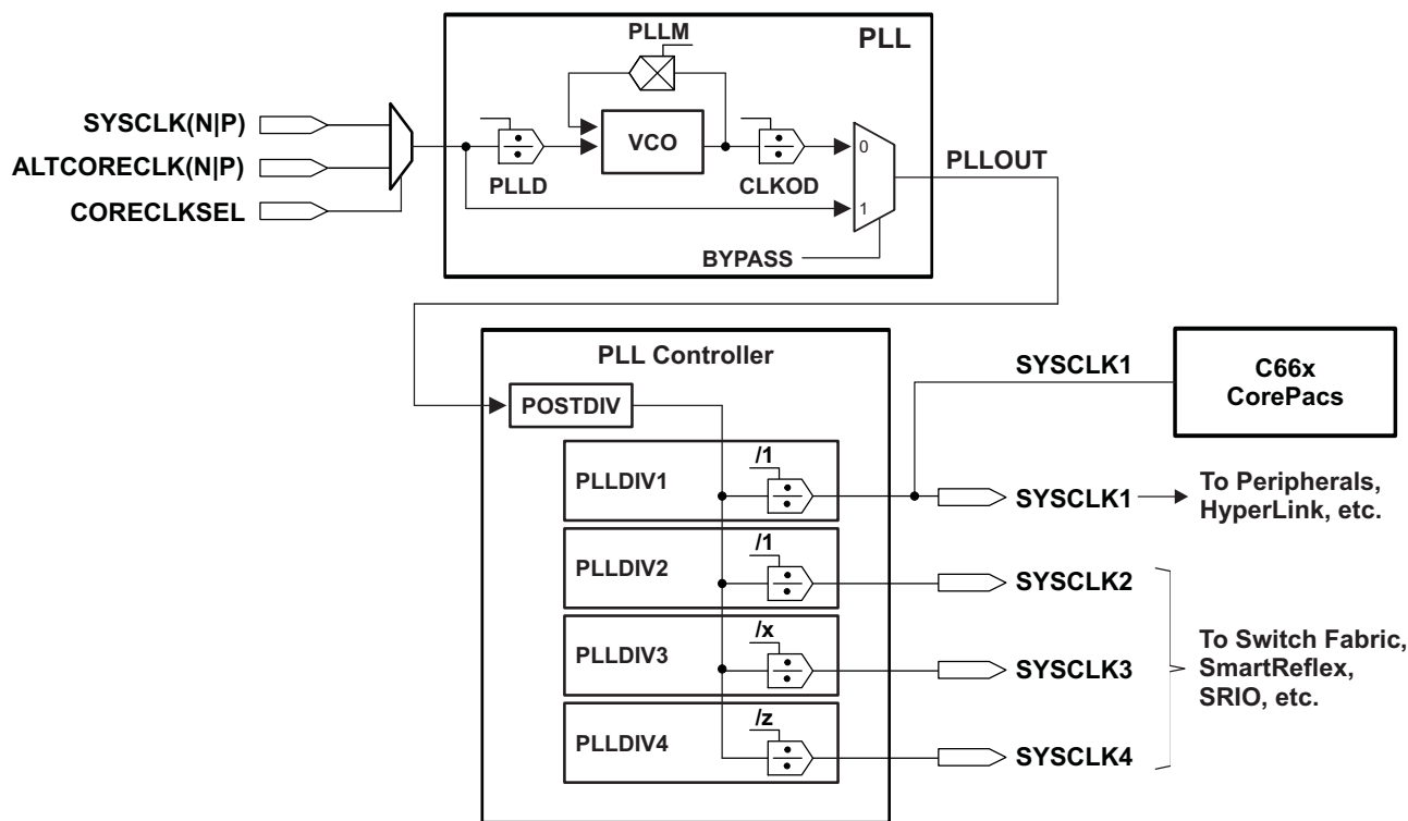
Figure 10-7 Main PLL and PLL Controller
