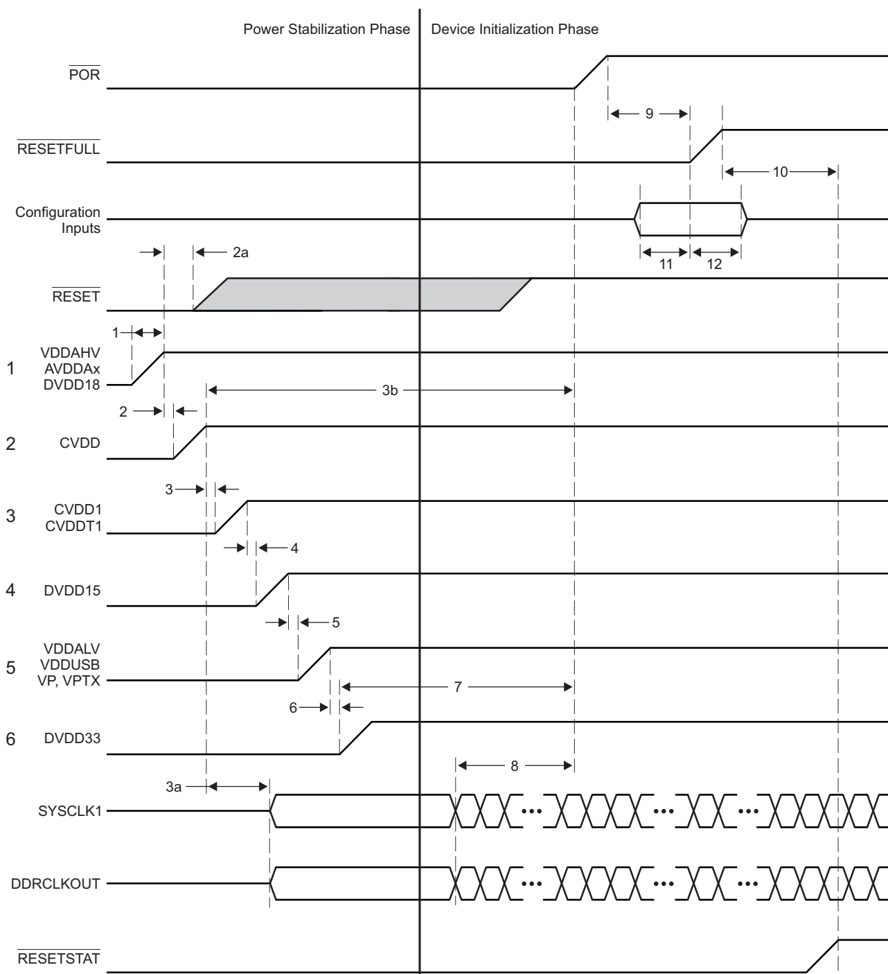
Figure 10-2 IO-Before-Core Power Sequencing
