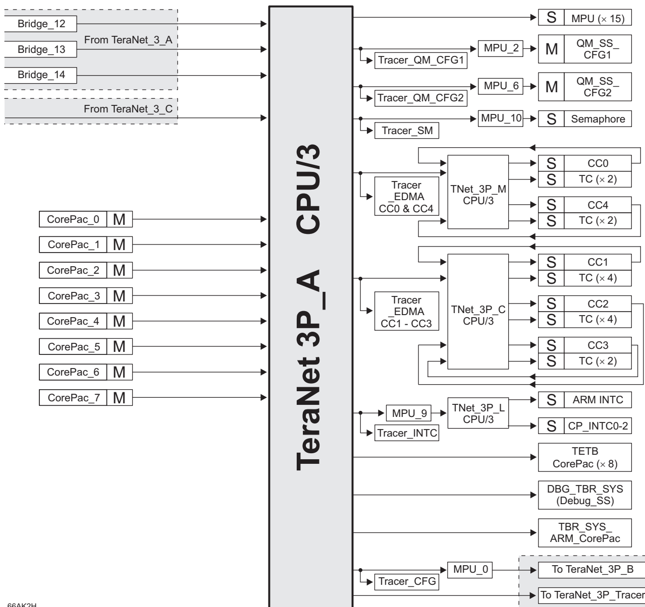
Figure 7-5 TeraNet 3P_A
