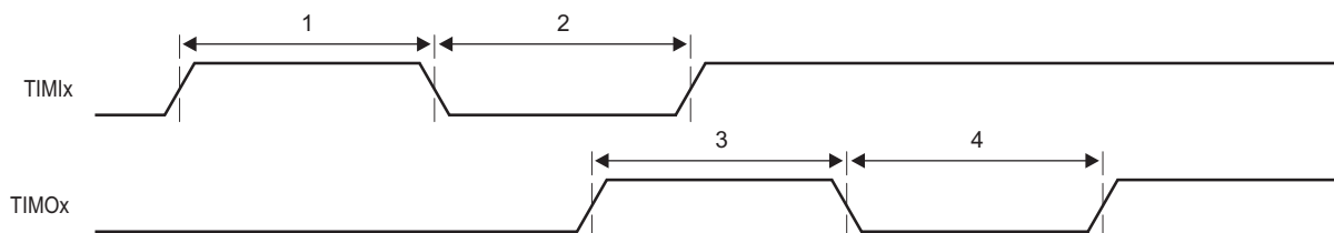
Figure 10-51 Timer Timing
