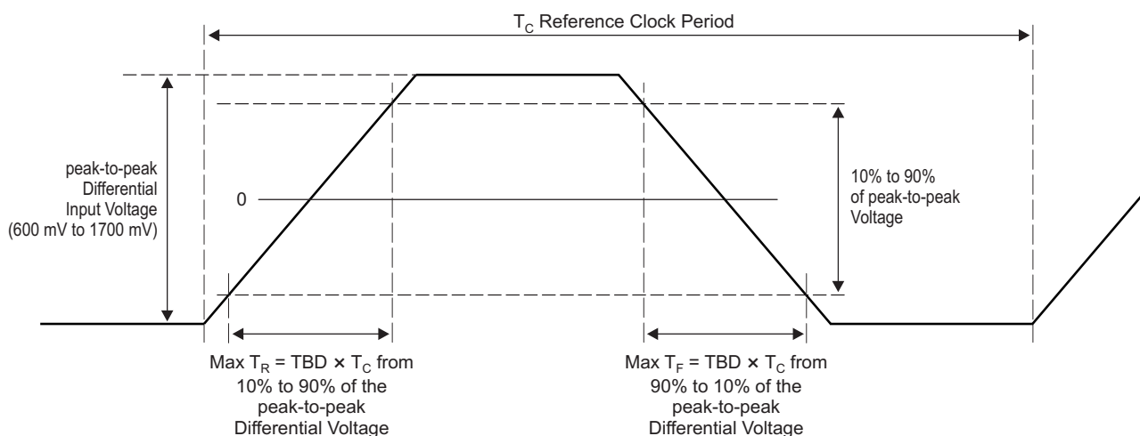
Figure 10-24 USBCLK Rise and Fall Times
