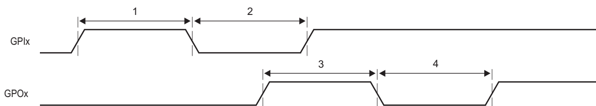
Figure 10-52 GPIO Timing
