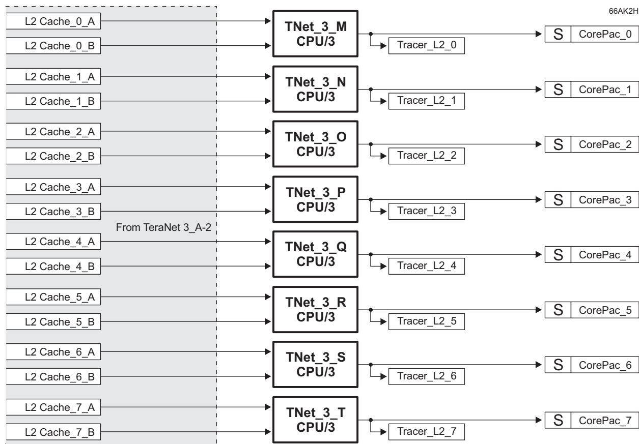
Figure 7-4 TeraNet C66x to SDMA
