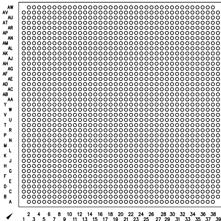
Figure 5-1 AAW 1517-PIN BGA Package (Bottom View)
