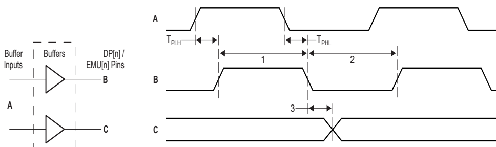
Figure 10-57 Trace Timing
