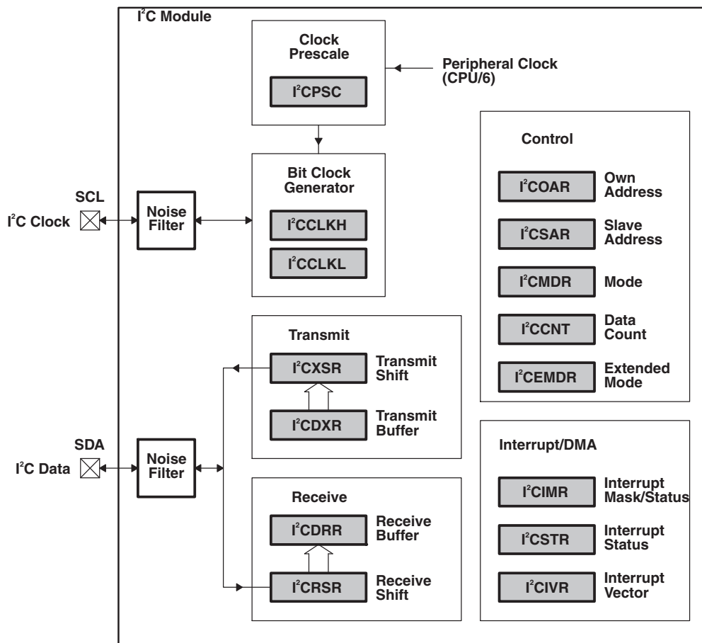
Figure 10-34 I 2 C Module Block Diagram
