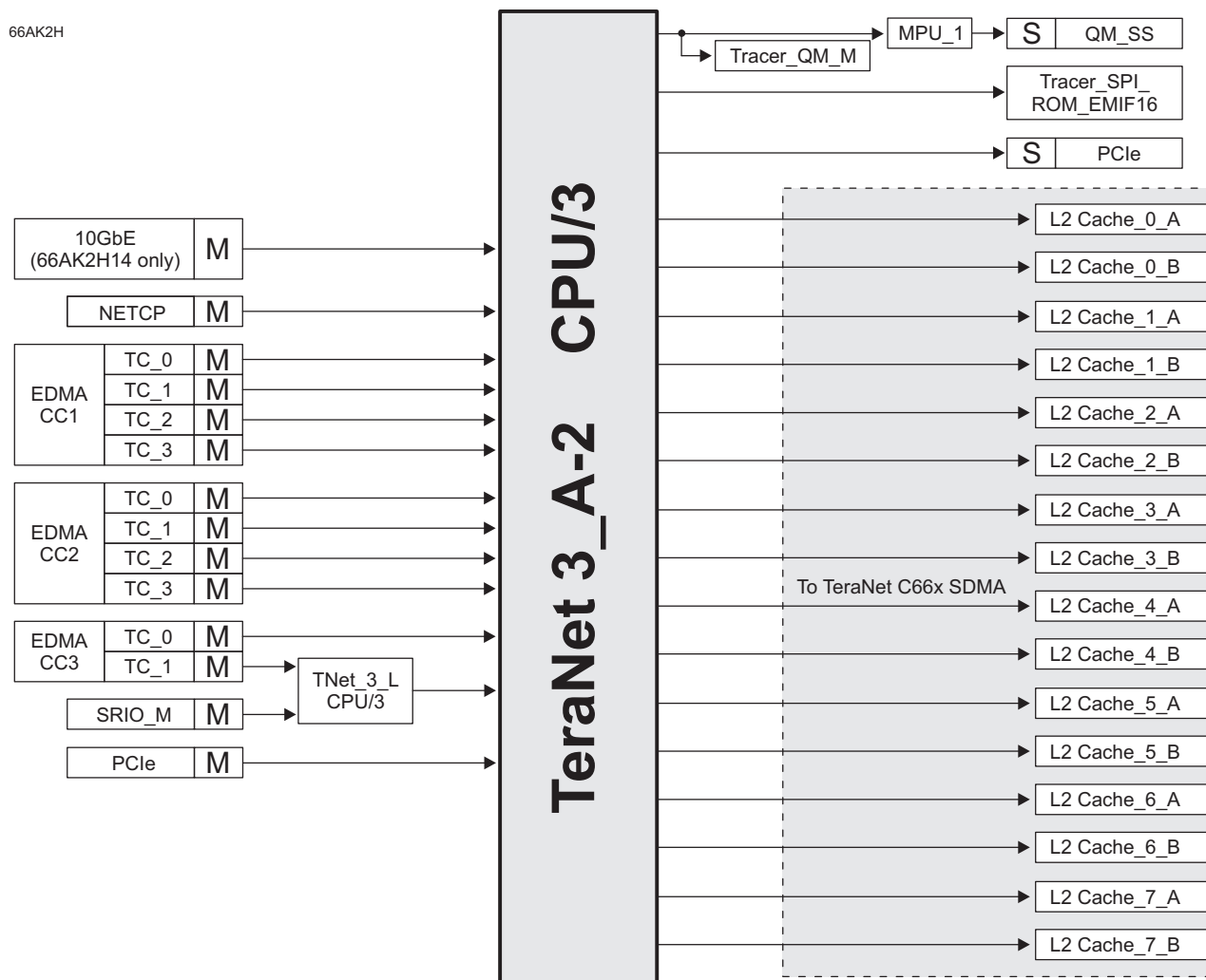
Figure 7-2 TeraNet 3_A-2
