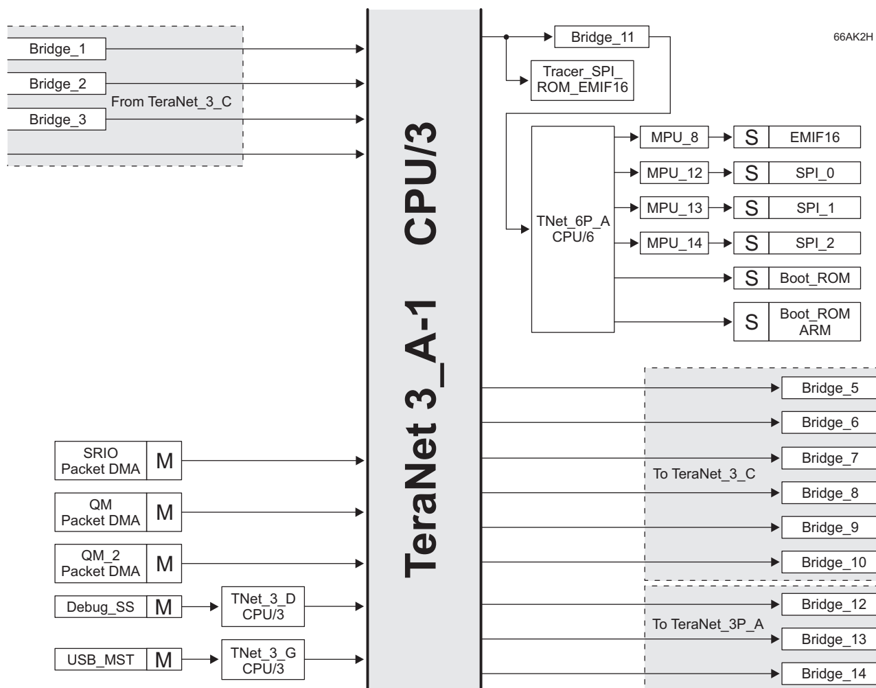
Figure 7-1 TeraNet 3_A-1
