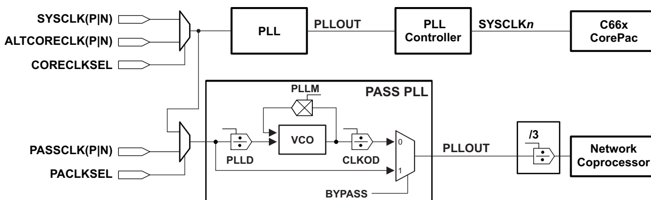
Figure 10-29 PASS PLL Block Diagram
