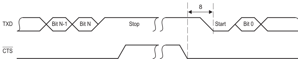
Figure 10-43 UART CTS (Clear-to-Send Input) — Autoflow Timing Waveform
