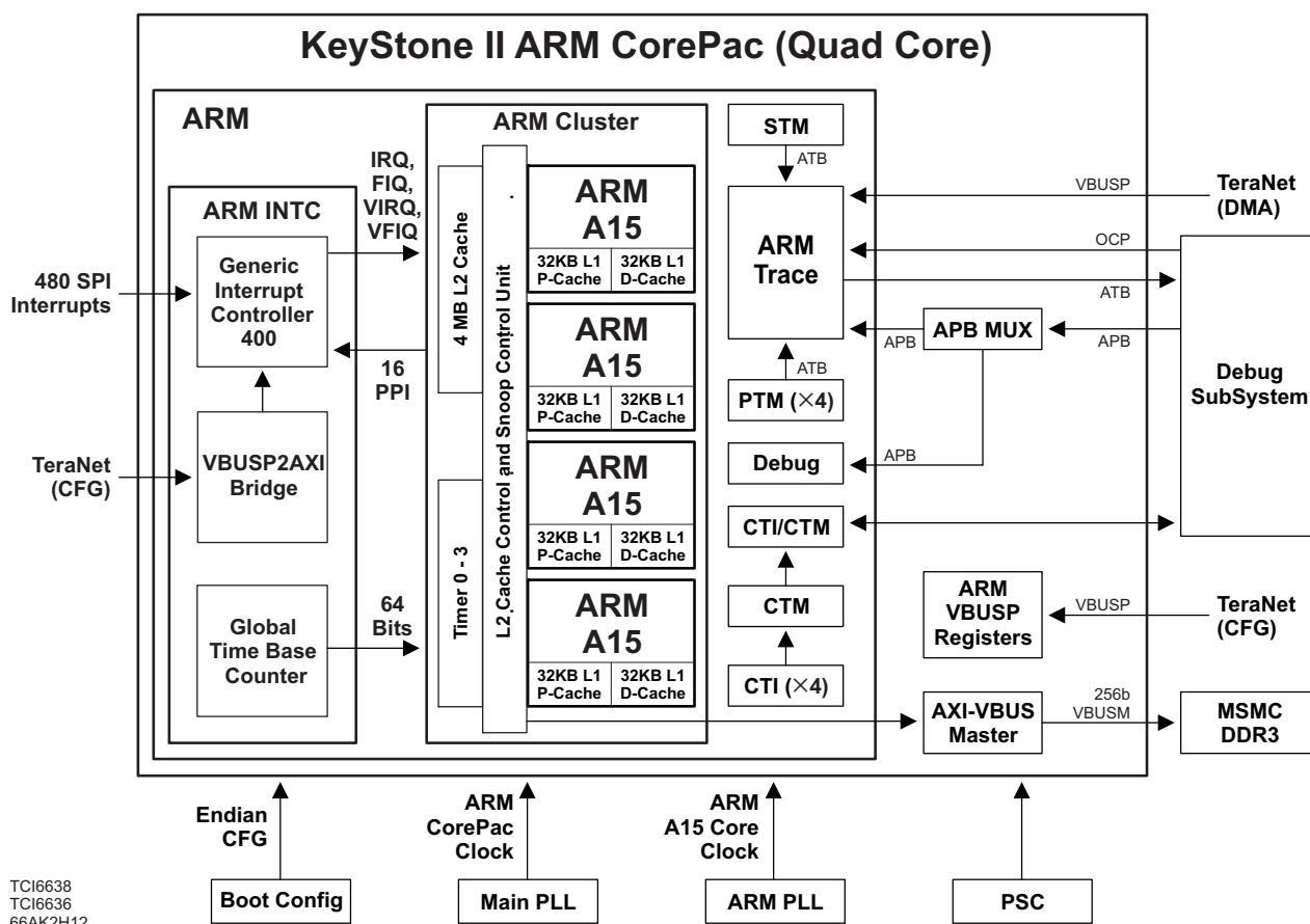
Figure 4-1 66AK2H12 ARM CorePac Block Diagram
