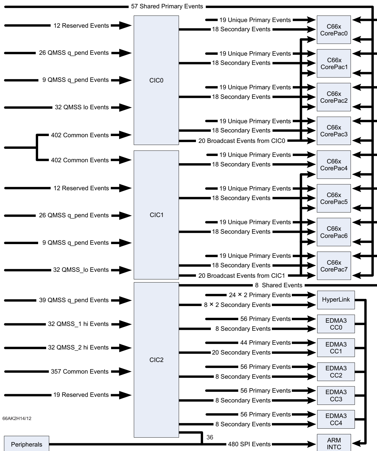
Figure 6-4 66AK2H14/12 Interrupt Topology
