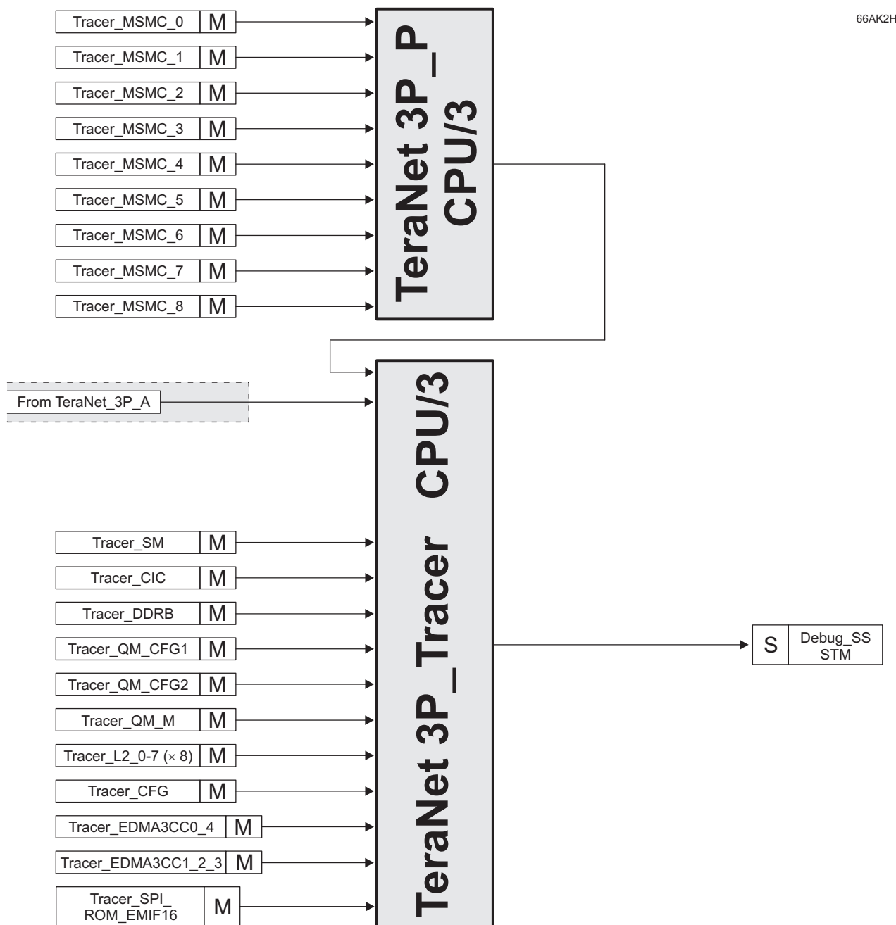
Figure 7-8 TeraNet 3P_Tracer
