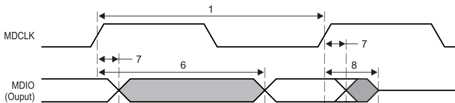
Figure 10-50 MDIO Output Timing
