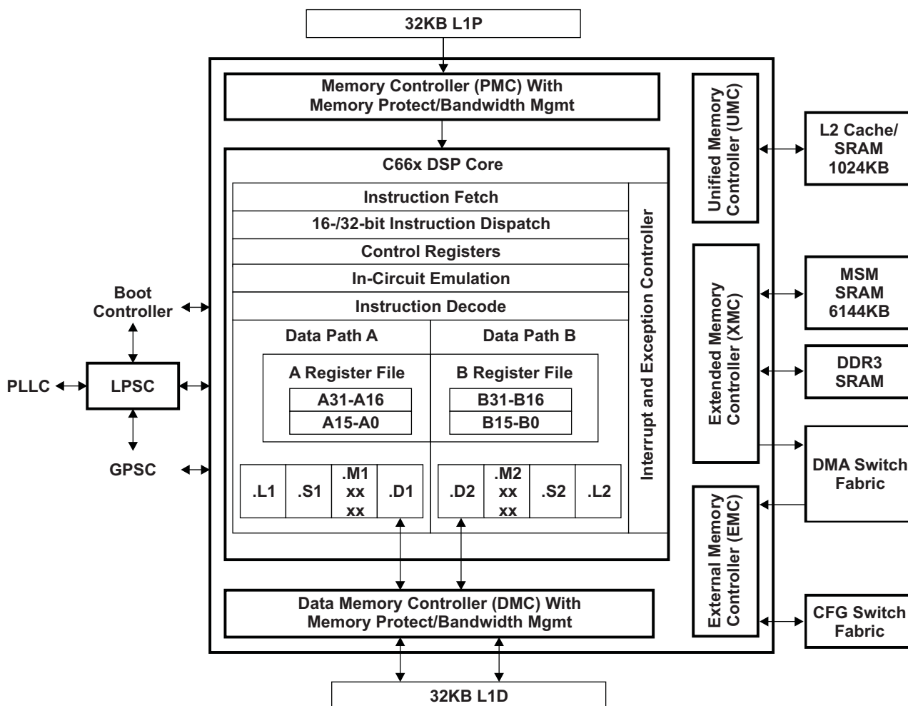
Figure 3-1 C66x CorePac Block Diagram
