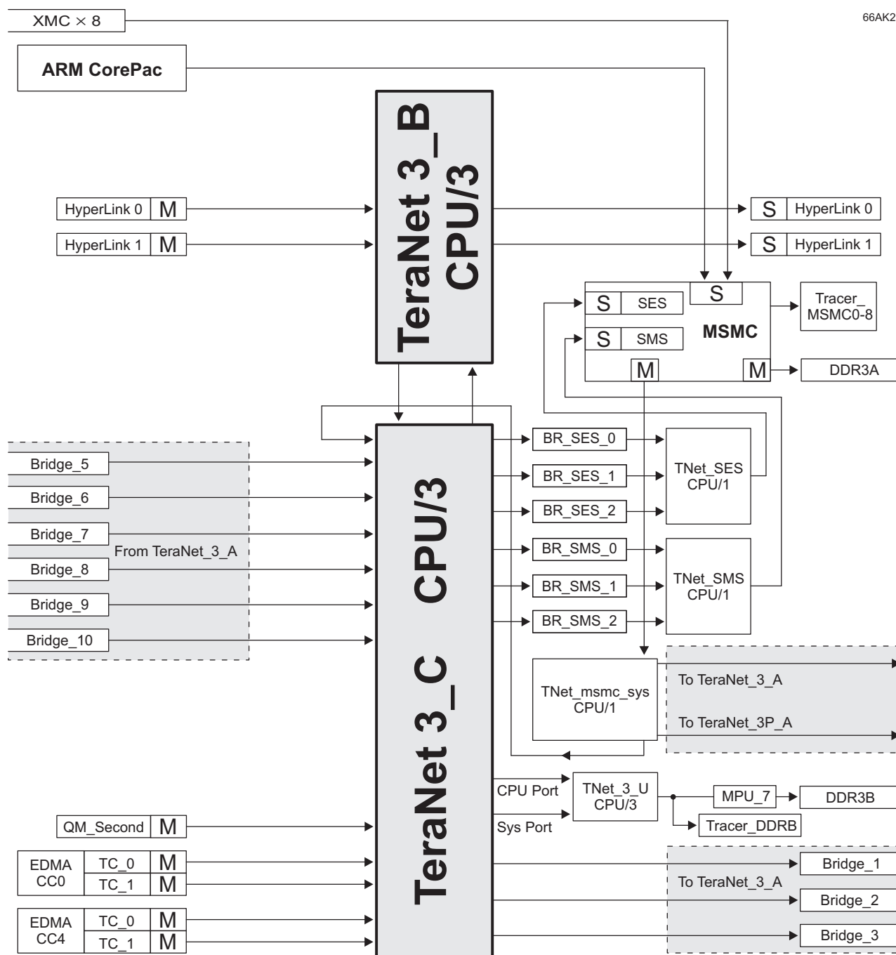
Figure 7-3 TeraNet 3_C
