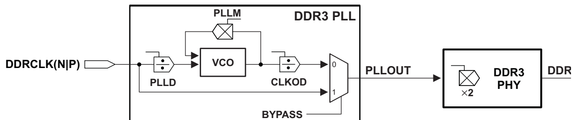
Figure 10-25 DDR3A PLL and DDR3B PLL Block Diagram
