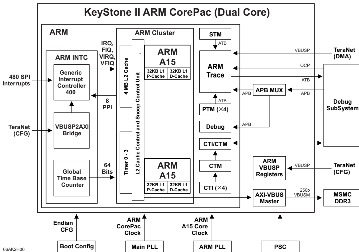
Figure 4-2 66AK2H06 ARM CorePac Block Diagram
