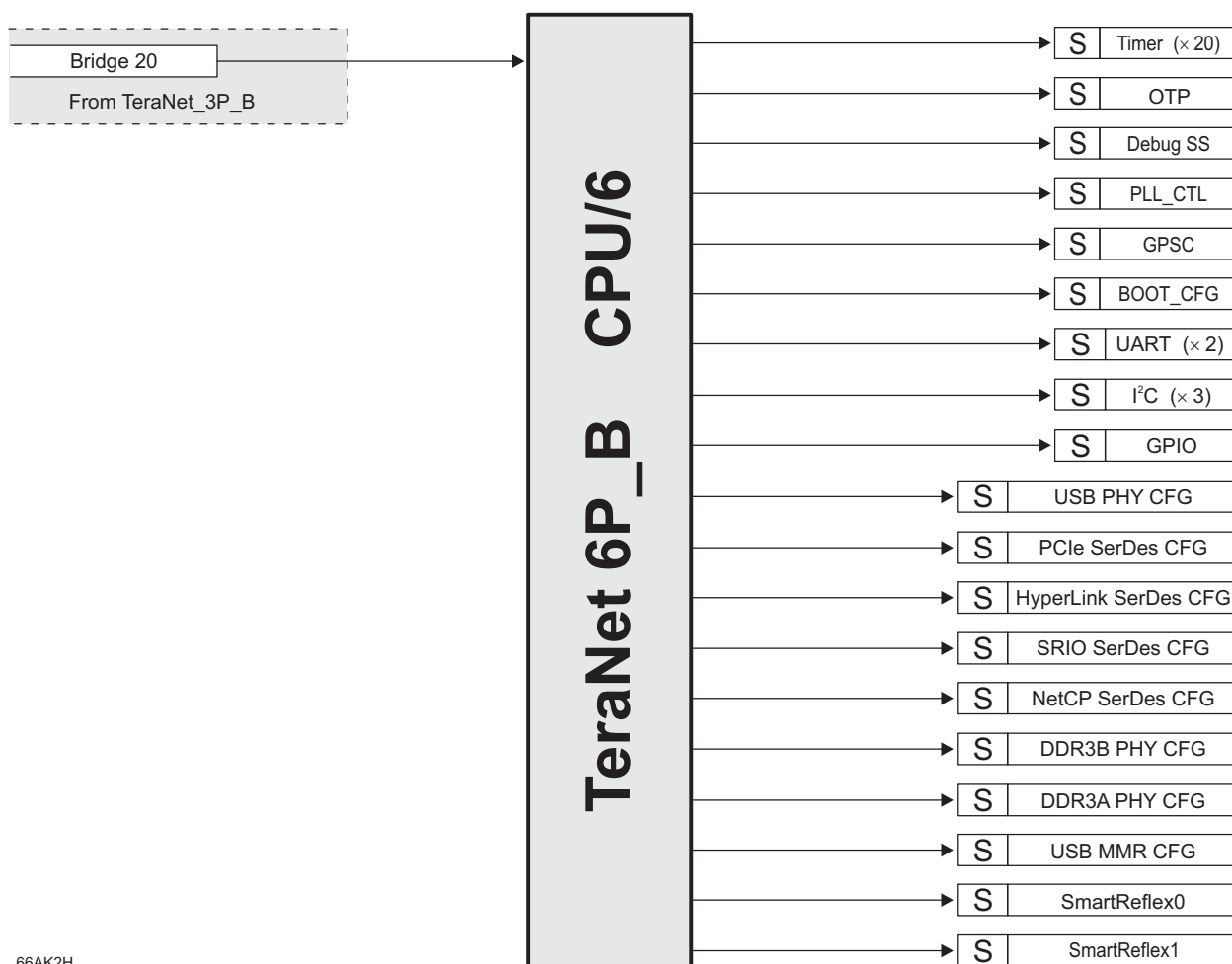
Figure 7-7 TeraNet 6P_B
