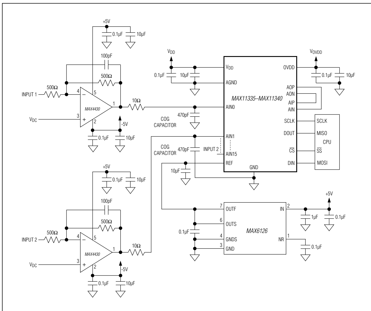
Figure 13. Typical Application Circuit
