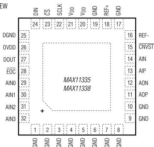
TQFN 4 CHANNEL
