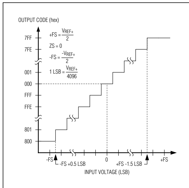
Figure 5. Bipolar Transfer Function for 12-Bit Resolution
