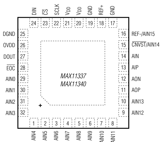
TQFN 16 CHANNEL
