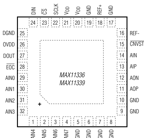
TQFN 8 CHANNEL
