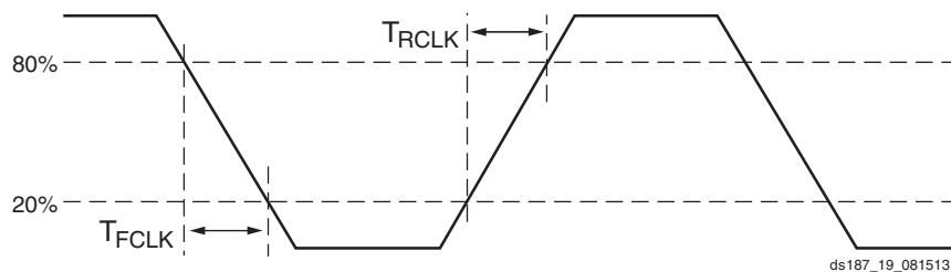
Figure 22: Reference Clock Timing Parameters
