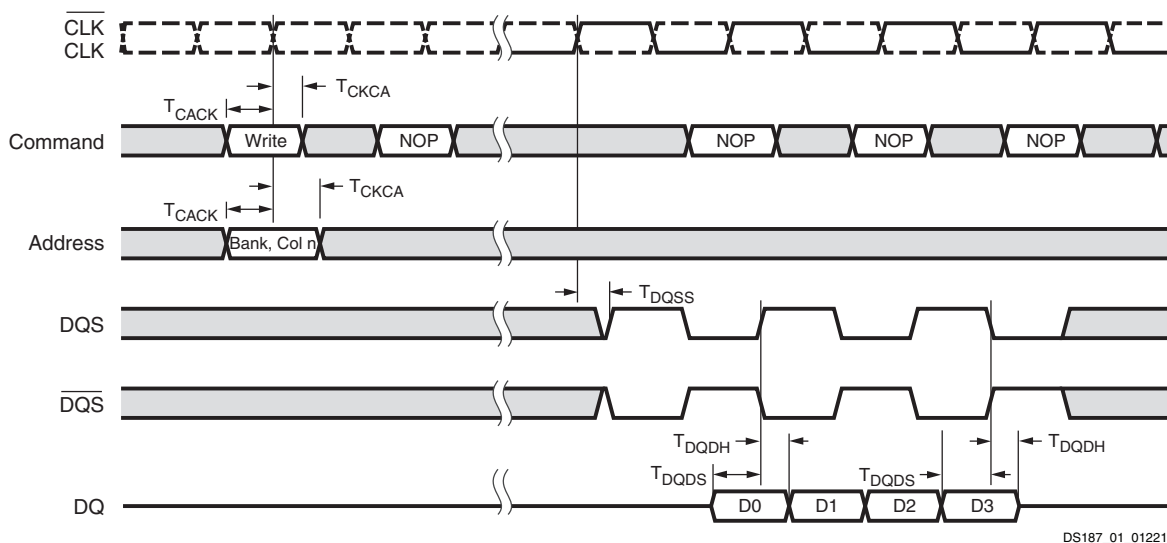
Figure 2: DDR Output Timing Diagram
