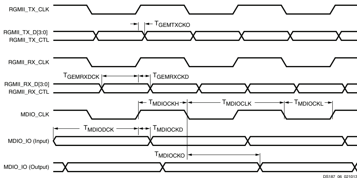
Figure 7: RGMII Interface Timing Diagram
