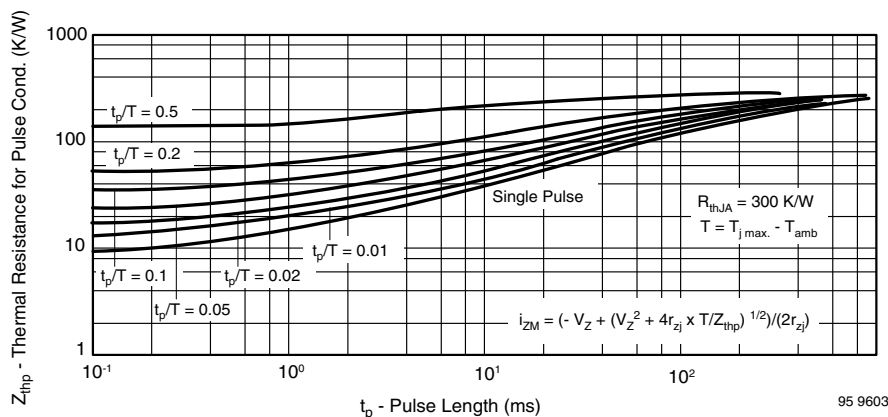
Fig. 11 - Thermal Response
