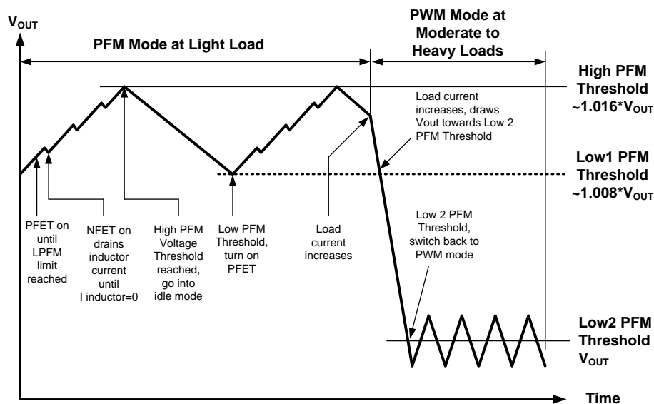
Figure 25. PFM vs PWM Operation
