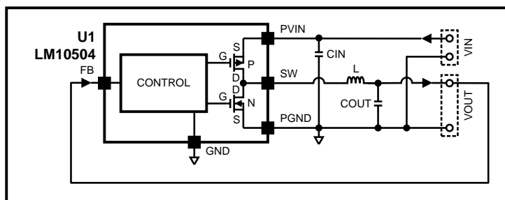
Figure 24. Buck Functional Diagram
