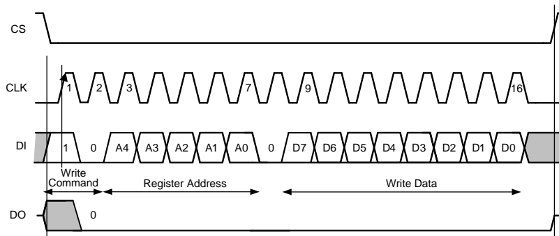
Figure 22. SPI Interface Write
