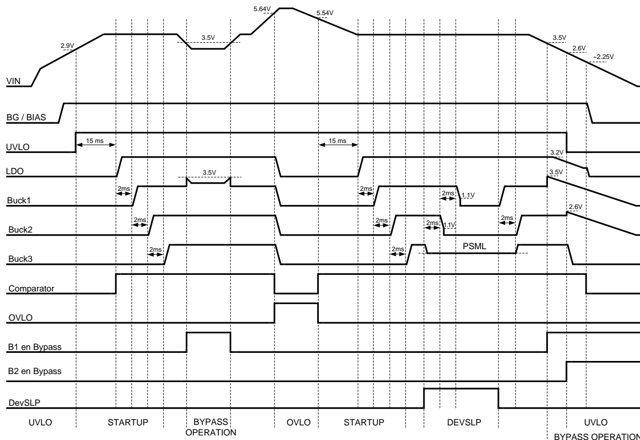
Figure 26. Operating Modes
