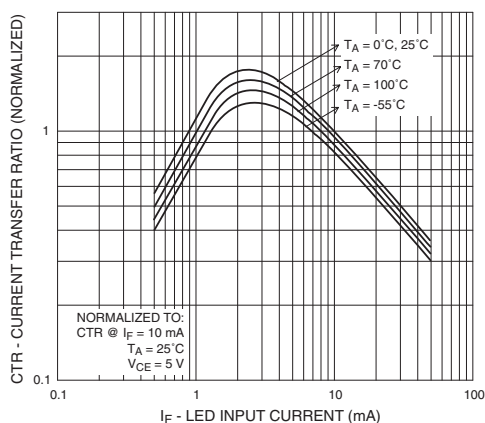
Fig. 1 Output Current vs. Input Current
