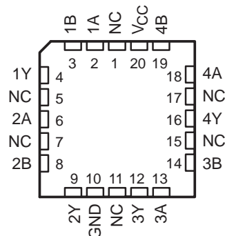
SN54HCT08 . . . FK PACKAGE (TOP VIEW)
