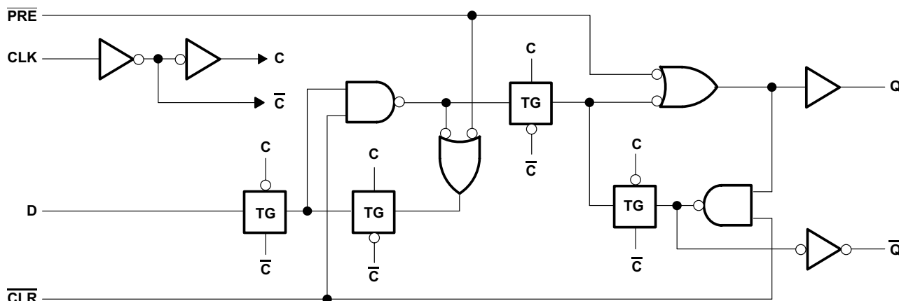
Figure 3. Logic Diagram (Positive Logic)
