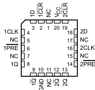
FK Package 20-Pin LCCC Top View
