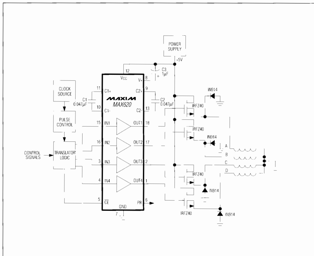
Figure 5. Four-Phase Stepper Motor Drive System
