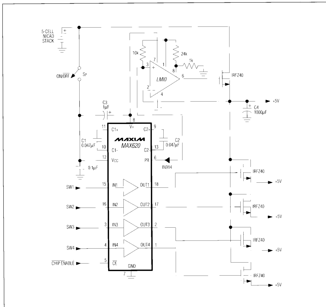
Figure 6. Logic-Controlled, +5V Regulated Power Distribution System
