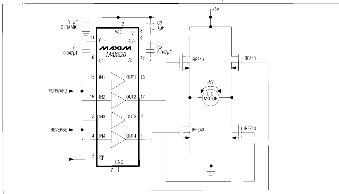
Figure 4. H-Bridge DC Motor Controller
