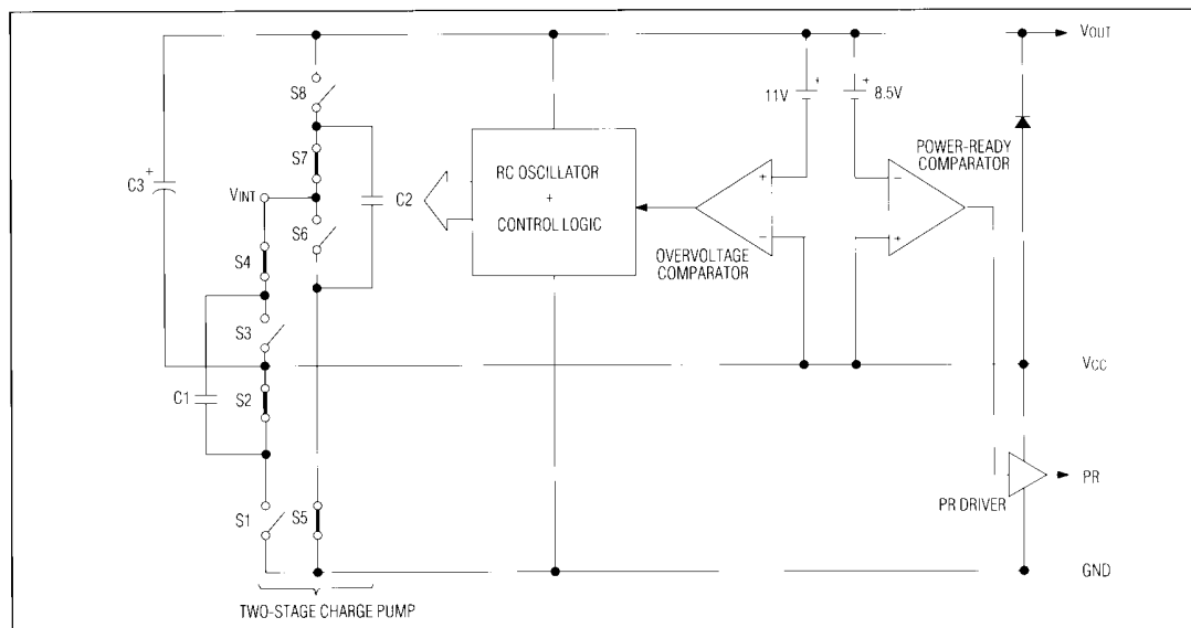
Figure 2. MAX620/MAX621 Charge Pump Block Diagram
