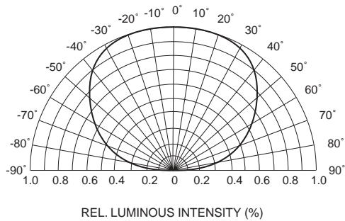
Fig.4 Radiation Diagram
