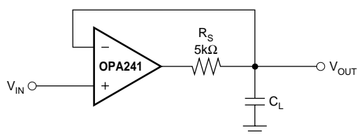
FIGURE 4. Series Resistor in Unity Gain Configuration Improves Capacitive Load Drive.
