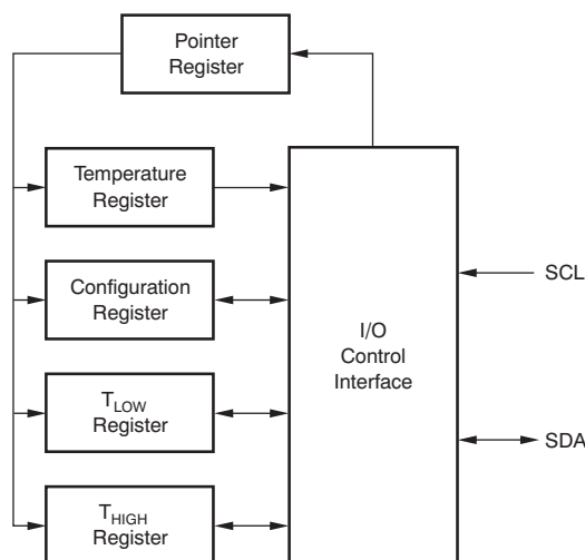
Figure 15. Internal Register Structure
