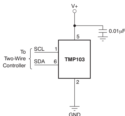
Figure 11. Typical Connections
