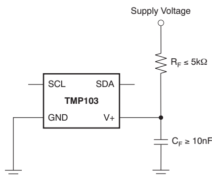
Figure 14. Noise Reduction
