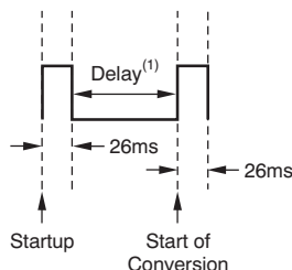
Figure 13. Conversion Start
