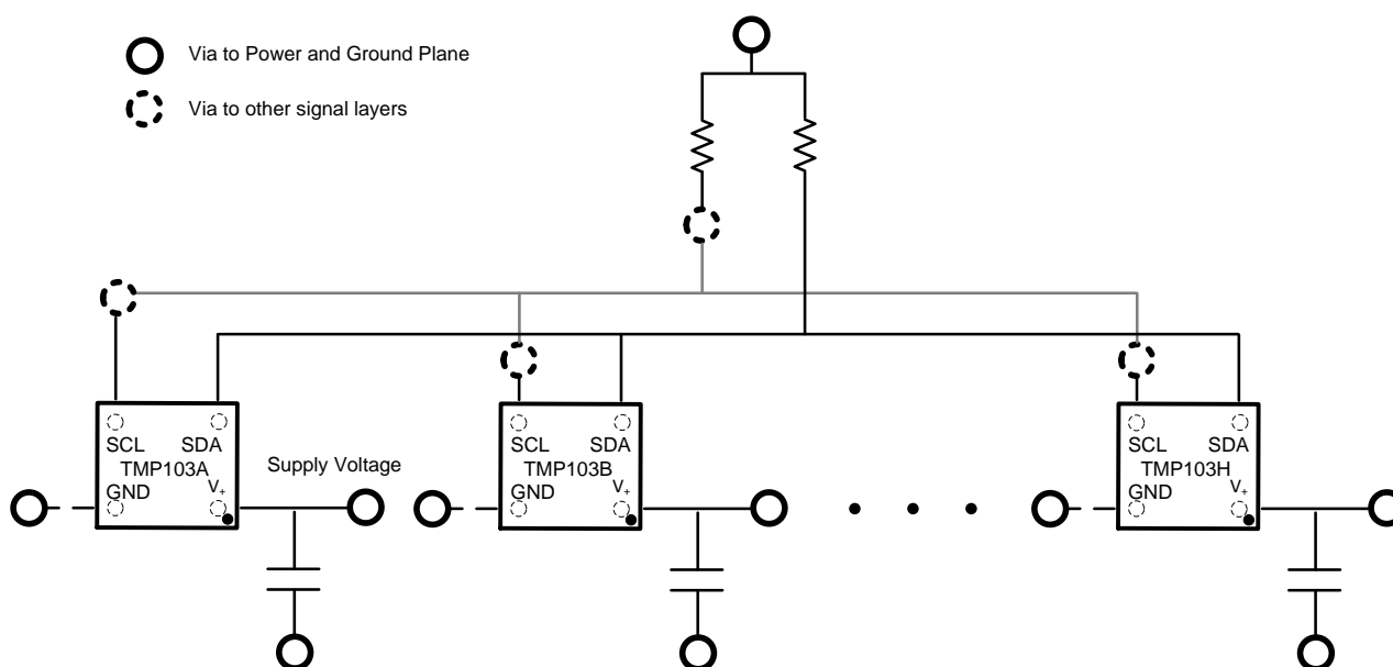
Figure 18. Recommended Layout Example
