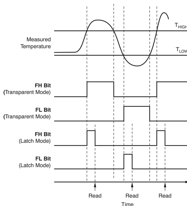
Figure 12. Temperature Flag Functional Diagram
