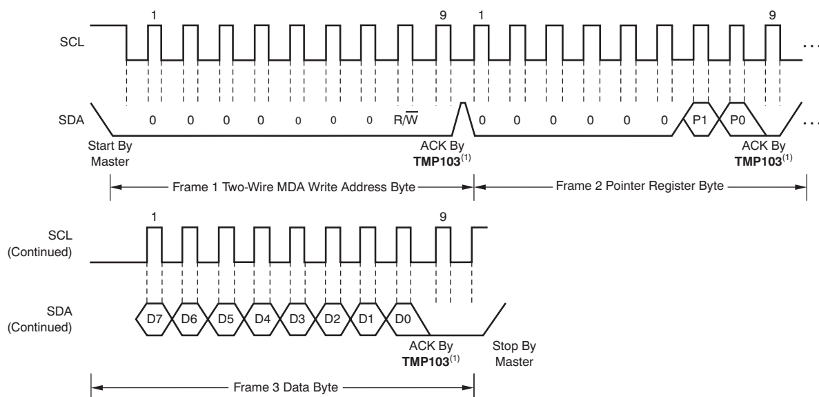
Figure 4. Two-Wire Timing Diagram MDA Write Word Format
