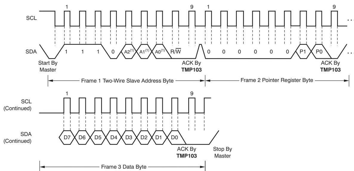
Figure 2. Two-Wire Timing Diagram for Write Word Format
