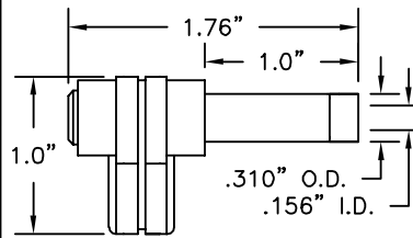
P/N 9309 Shrouded Right Angle Banana Socket Fits Simpson and Triplet
