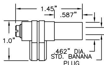
P/N 9301 Shrouded Right Angle Banana Plug Fits Amprobe and some Beckman
